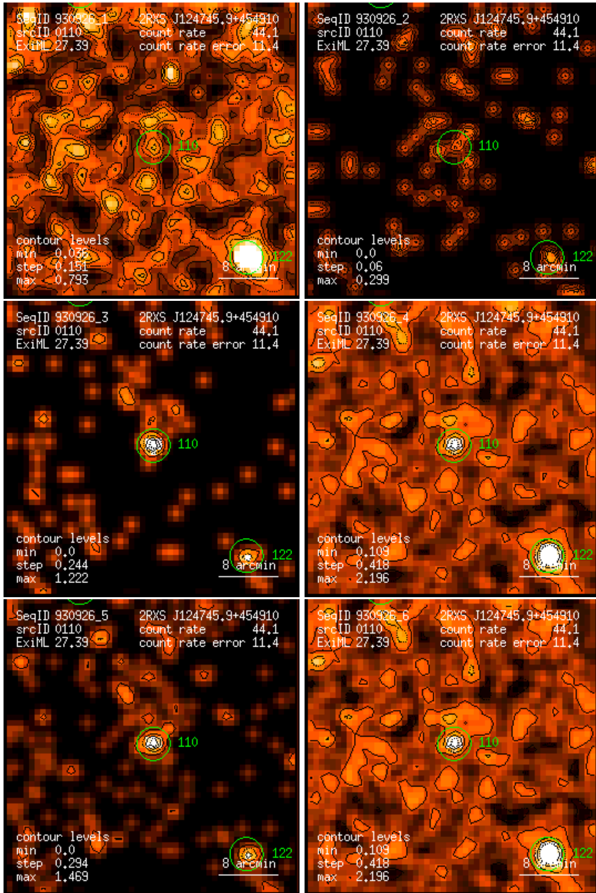
Figure 110: RASS 930926: detection 0110: band rate images, Gaussian filter: (1) PSPC channels 11 – 41, (2) 52 – 90, (3) 91 – 201, (4) 11 – 235, (5) 52 – 201, (6) 11 – 201. Broad band rates in counts/ks. Band rate contour levels in counts/ks/arcmin 2 .
