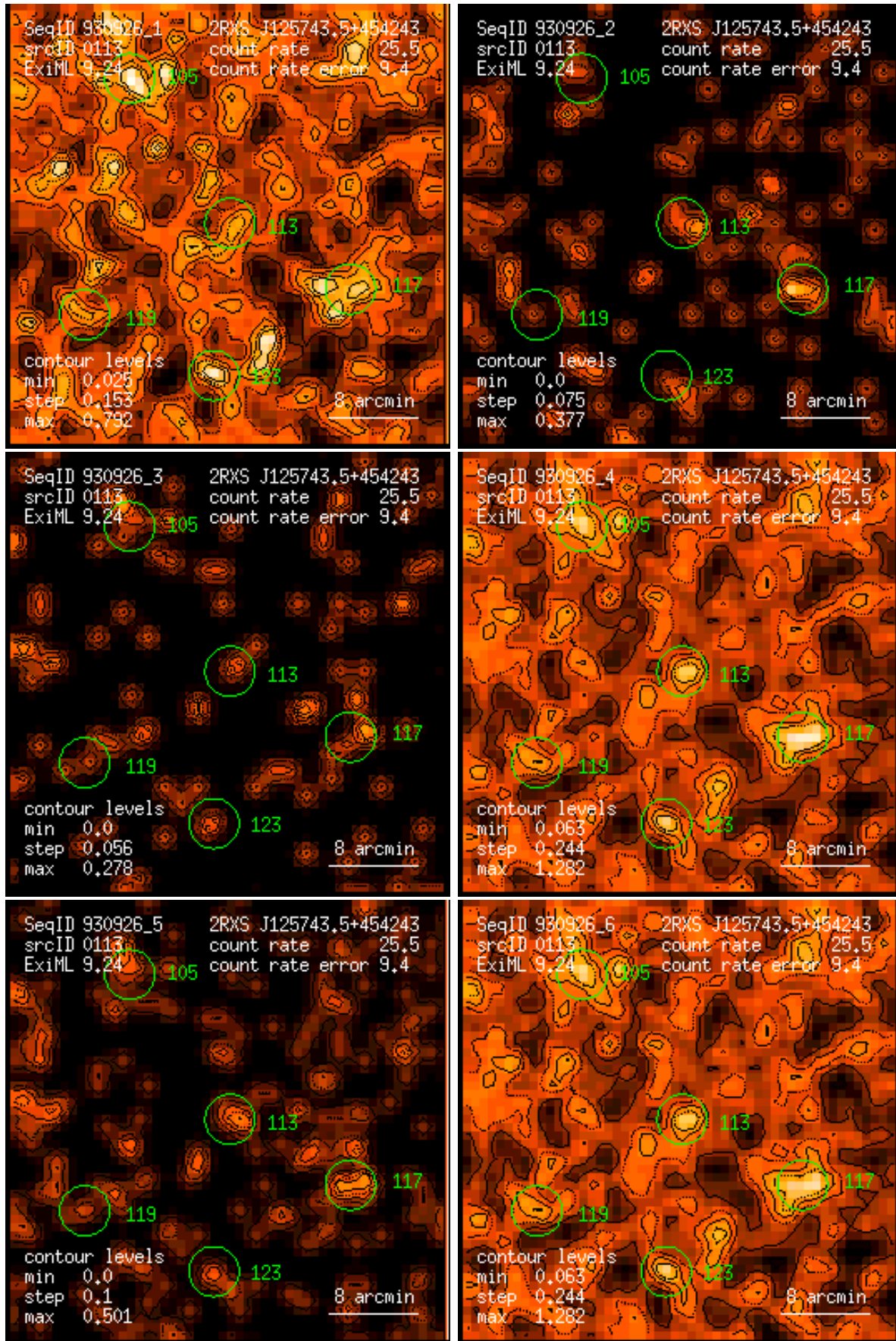
Figure 113: RASS 930926: detection 0113: band rate images, Gaussian filter: (1) PSPC channels 11 – 41, (2) 52 – 90, (3) 91 – 201, (4) 11 – 235, (5) 52 – 201, (6) 11 – 201. Broad band rates in counts/ks. Band rate contour levels in counts/ks/arcmin 2 .
