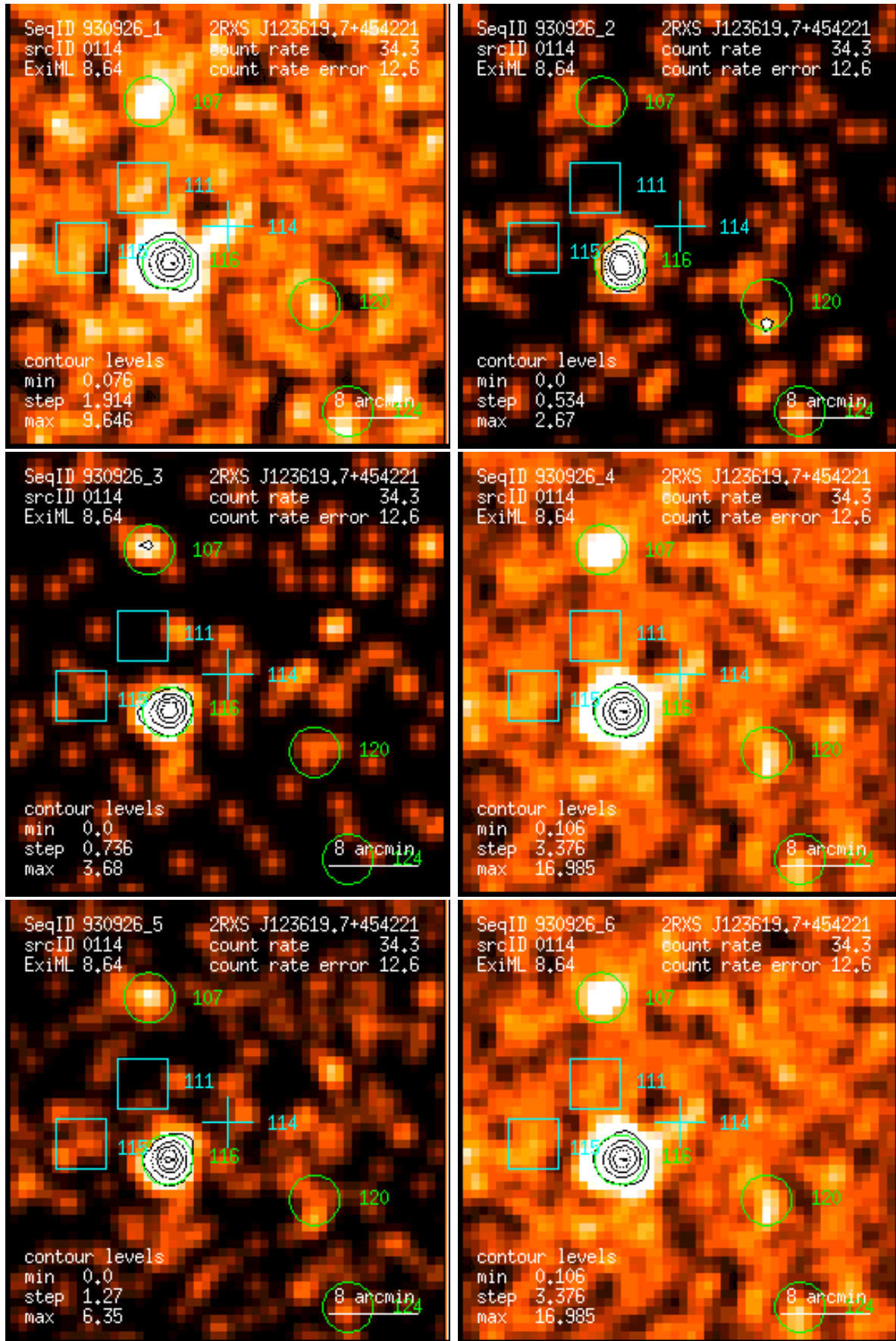
Figure 114: RASS 930926: detection 0114: band rate images, Gaussian filter: (1) PSPC channels 11 – 41, (2) 52 – 90, (3) 91 – 201, (4) 11 – 235, (5) 52 – 201, (6) 11 – 201. Broad band rates in counts/ks. Band rate contour levels in counts/ks/arcmin 2 .
