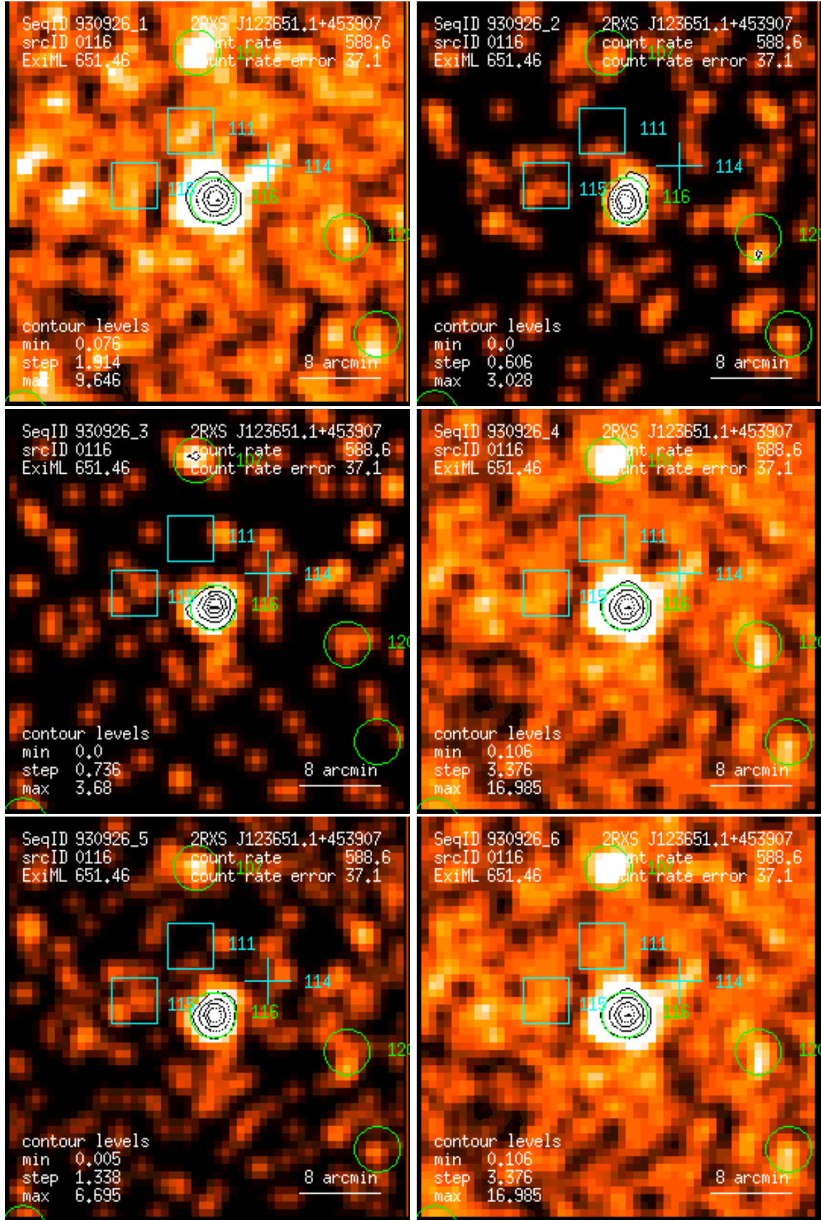
Figure 116: RASS 930926: detection 0116: band rate images, Gaussian filter: (1) PSPC channels 11 – 41, (2) 52 – 90, (3) 91 – 201, (4) 11 – 235, (5) 52 – 201, (6) 11 – 201. Broad band rates in counts/ks. Band rate contour levels in counts/ks/arcmin 2 .
