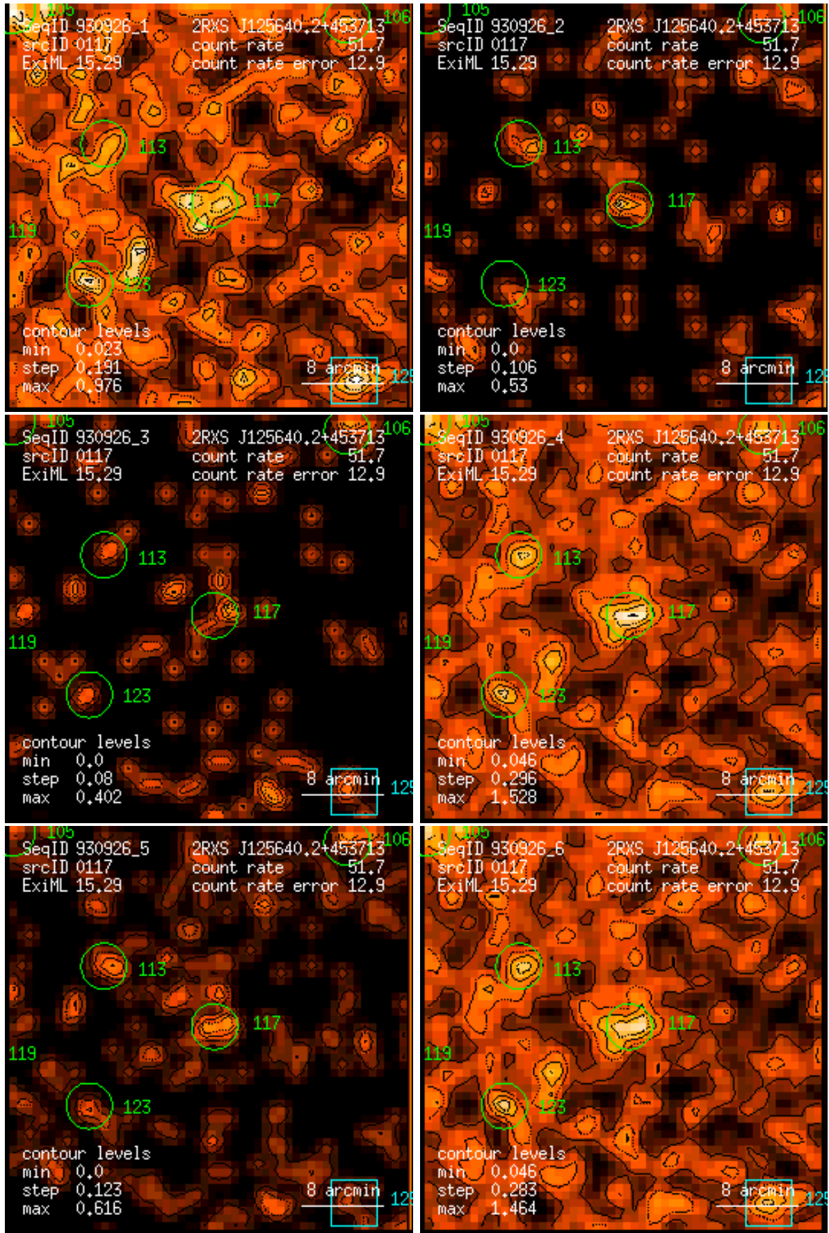
Figure 117: RASS 930926: detection 0117: band rate images, Gaussian filter: (1) PSPC channels 11 – 41, (2) 52 – 90, (3) 91 – 201, (4) 11 – 235, (5) 52 – 201, (6) 11 – 201. Broad band rates in counts/ks. Band rate contour levels in counts/ks/arcmin 2 .
