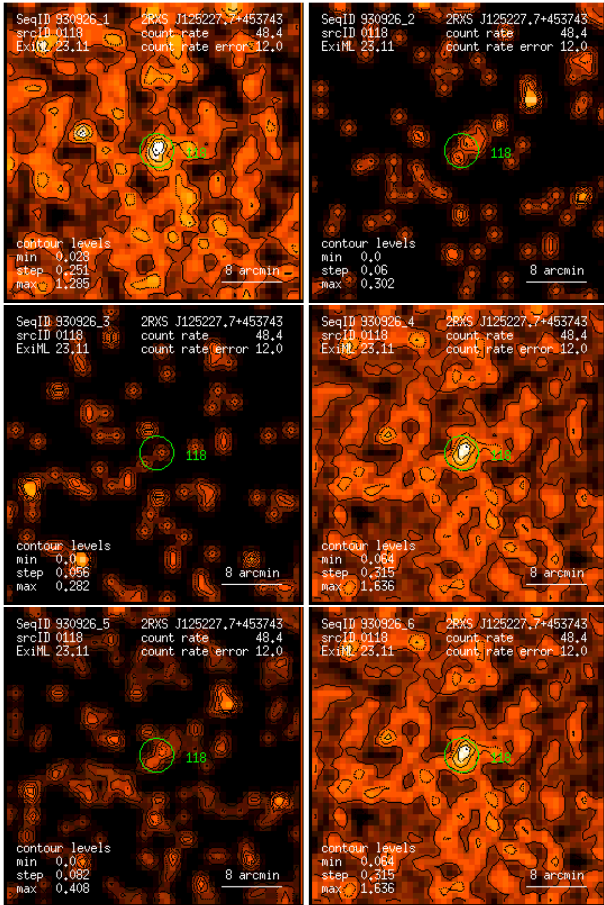
Figure 118: RASS 930926: detection 0118: band rate images, Gaussian filter: (1) PSPC channels 11 – 41, (2) 52 – 90, (3) 91 – 201, (4) 11 – 235, (5) 52 – 201, (6) 11 – 201. Broad band rates in counts/ks. Band rate contour levels in counts/ks/arcmin 2 .
