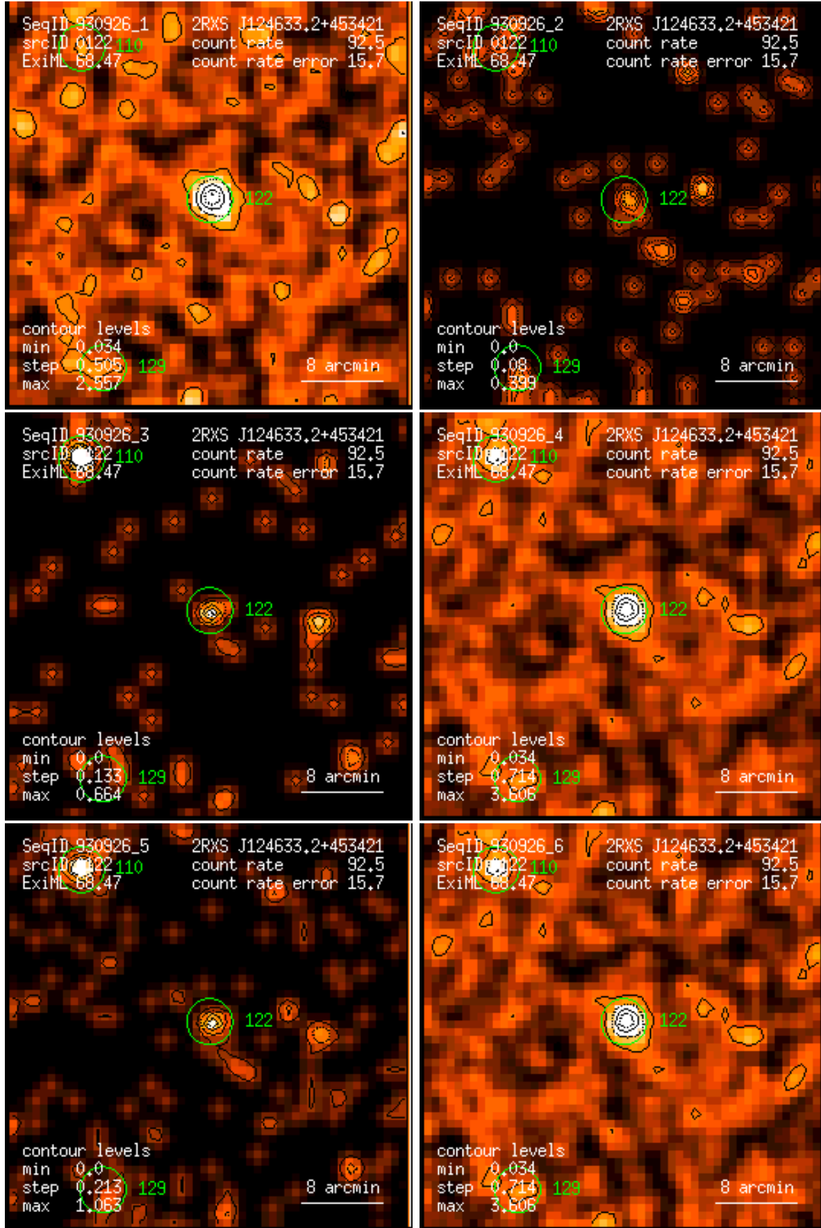
Figure 122: RASS 930926: detection 0122: band rate images, Gaussian filter: (1) PSPC channels 11 – 41, (2) 52 – 90, (3) 91 – 201, (4) 11 – 235, (5) 52 – 201, (6) 11 – 201. Broad band rates in counts/ks. Band rate contour levels in counts/ks/arcmin 2 .
