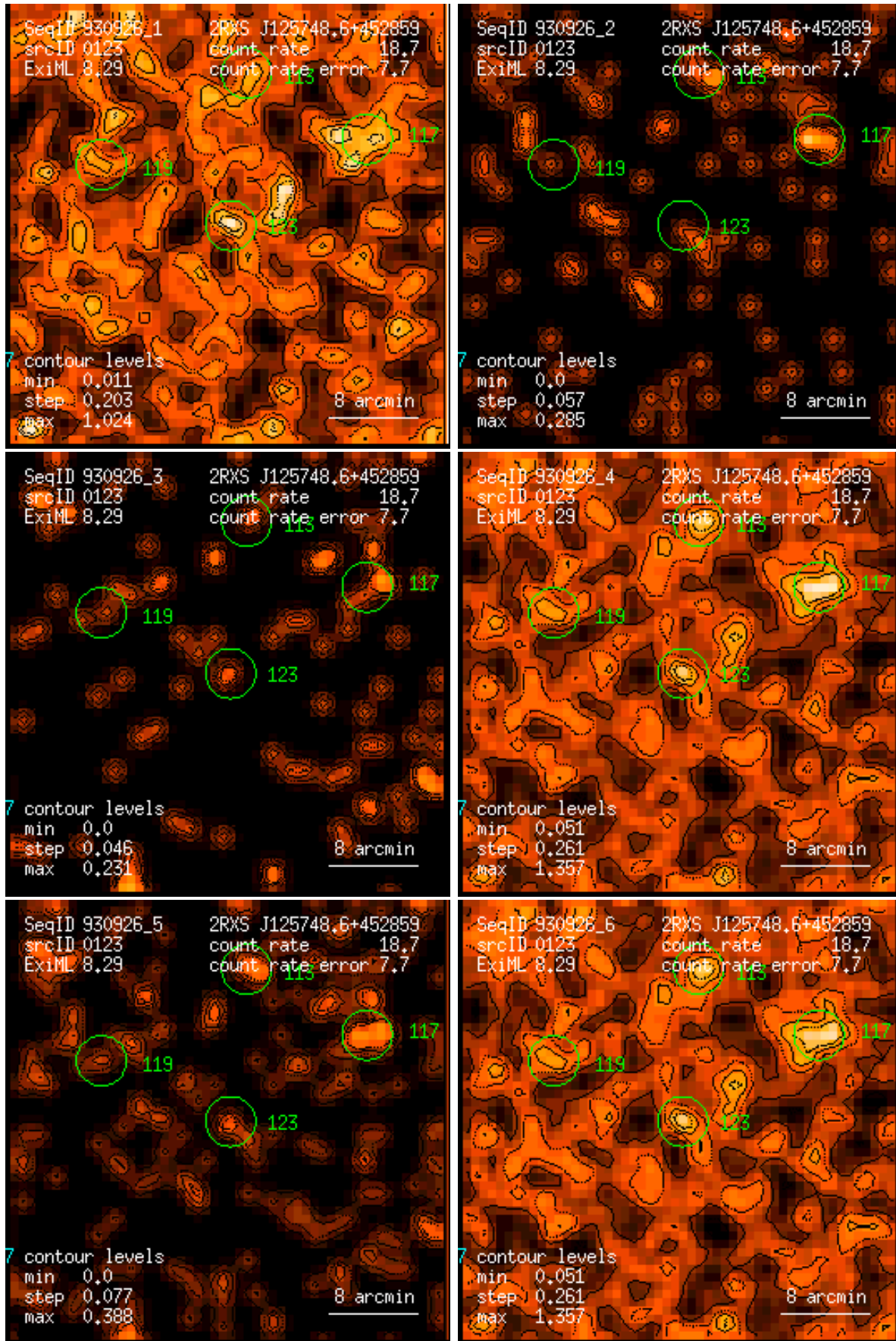
Figure 123: RASS 930926: detection 0123: band rate images, Gaussian filter: (1) PSPC channels 11 – 41, (2) 52 – 90, (3) 91 – 201, (4) 11 – 235, (5) 52 – 201, (6) 11 – 201. Broad band rates in counts/ks. Band rate contour levels in counts/ks/arcmin 2 .
