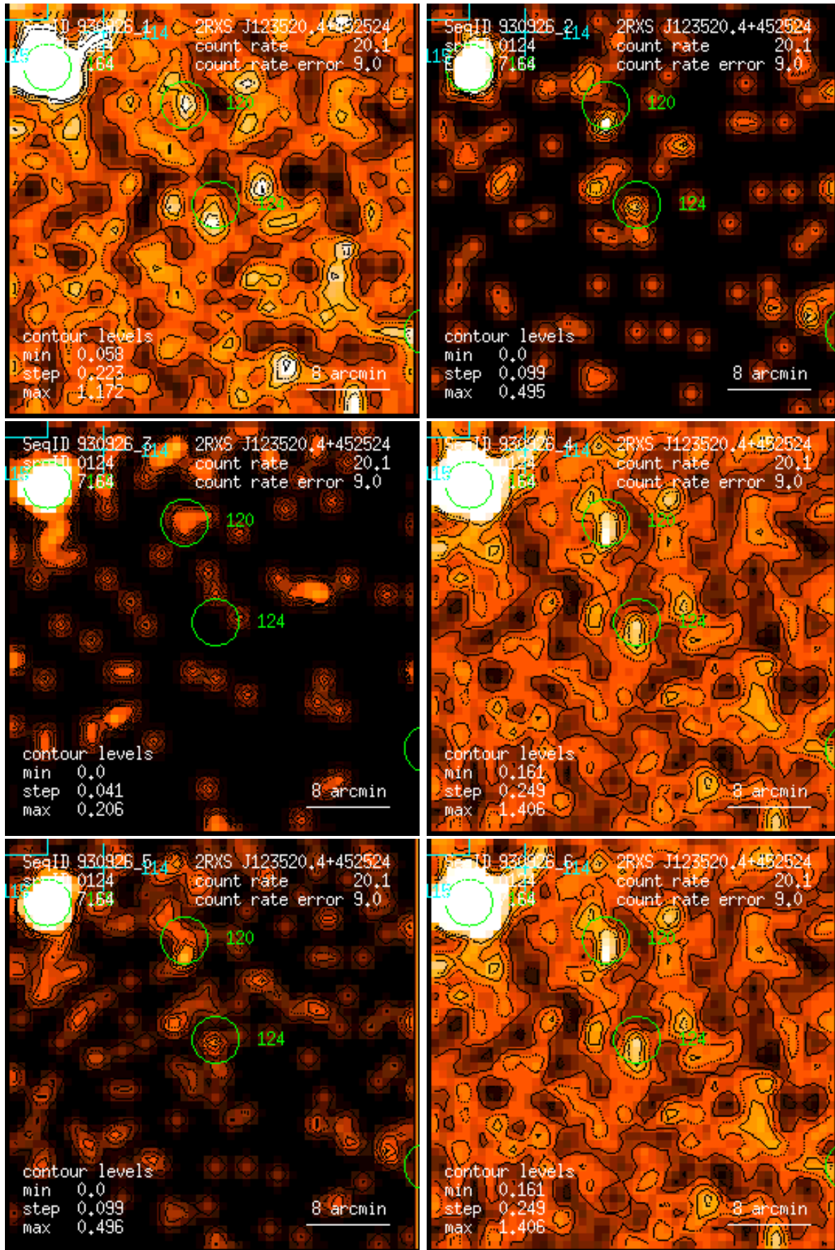
Figure 124: RASS 930926: detection 0124: band rate images, Gaussian filter: (1) PSPC channels 11 – 41, (2) 52 – 90, (3) 91 – 201, (4) 11 – 235, (5) 52 – 201, (6) 11 – 201. Broad band rates in counts/ks. Band rate contour levels in counts/ks/arcmin 2 .
