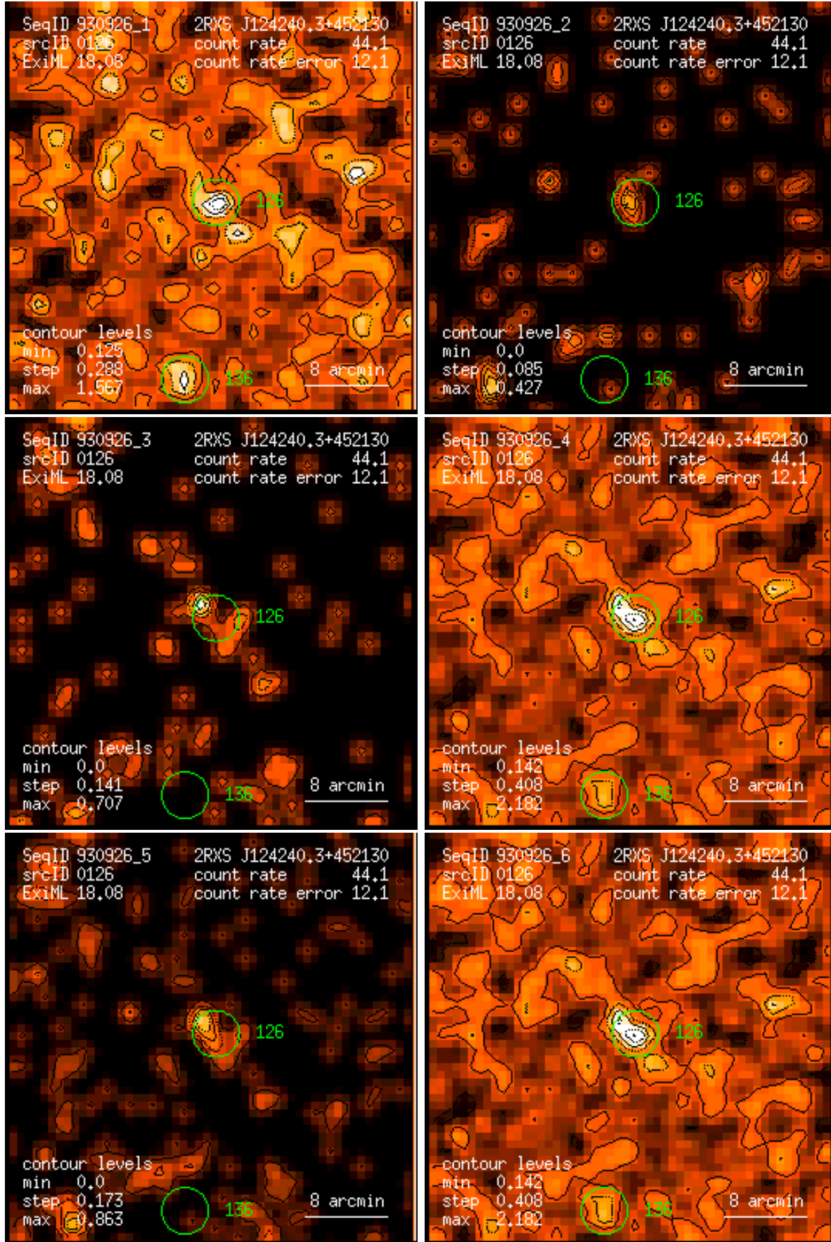
Figure 126: RASS 930926: detection 0126: band rate images, Gaussian filter: (1) PSPC channels 11 – 41, (2) 52 – 90, (3) 91 – 201, (4) 11 – 235, (5) 52 – 201, (6) 11 – 201. Broad band rates in counts/ks. Band rate contour levels in counts/ks/arcmin 2 .
