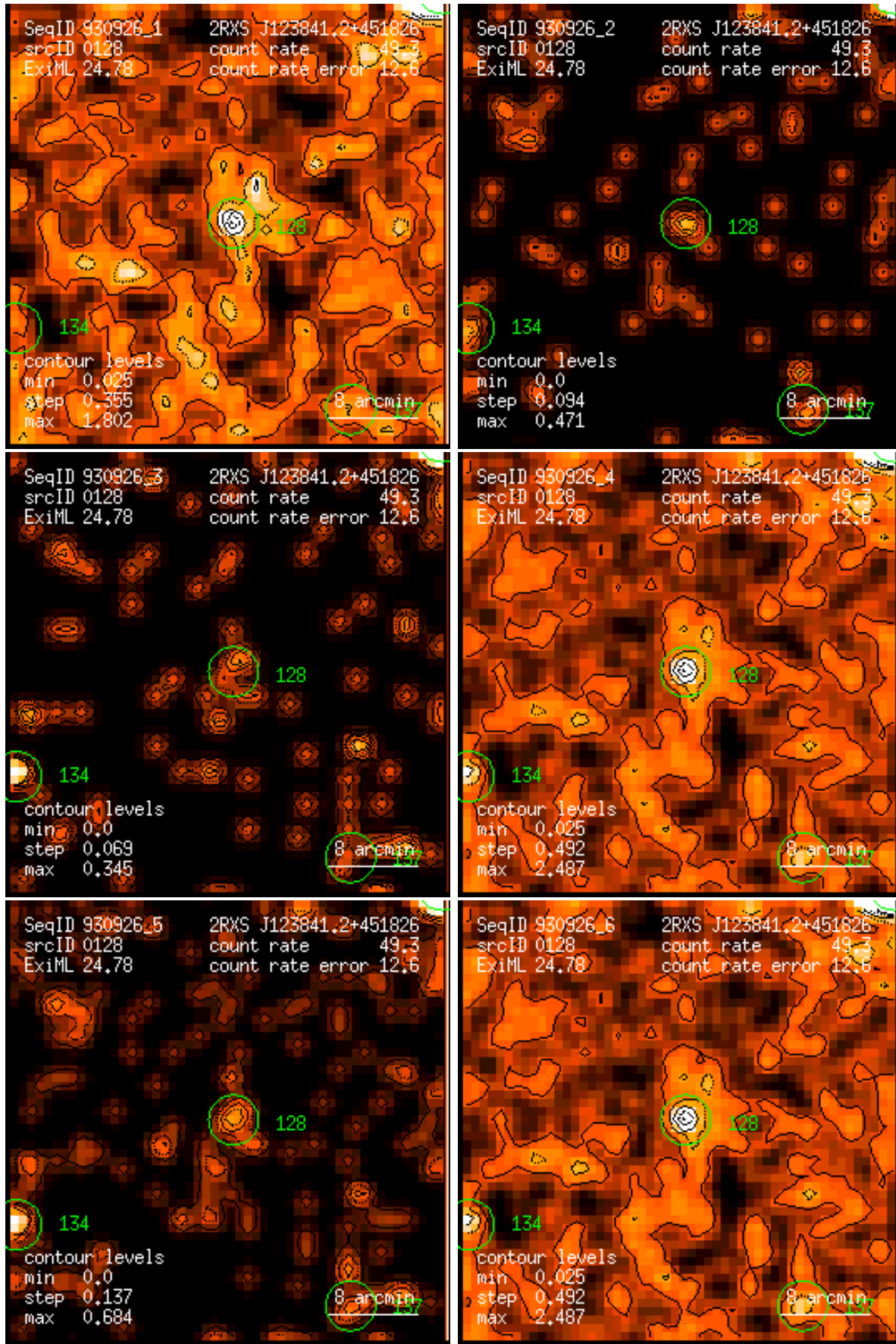
Figure 128: RASS 930926: detection 0128: band rate images, Gaussian filter: (1) PSPC channels 11 – 41, (2) 52 – 90, (3) 91 – 201, (4) 11 – 235, (5) 52 – 201, (6) 11 – 201. Broad band rates in counts/ks. Band rate contour levels in counts/ks/arcmin 2 .
