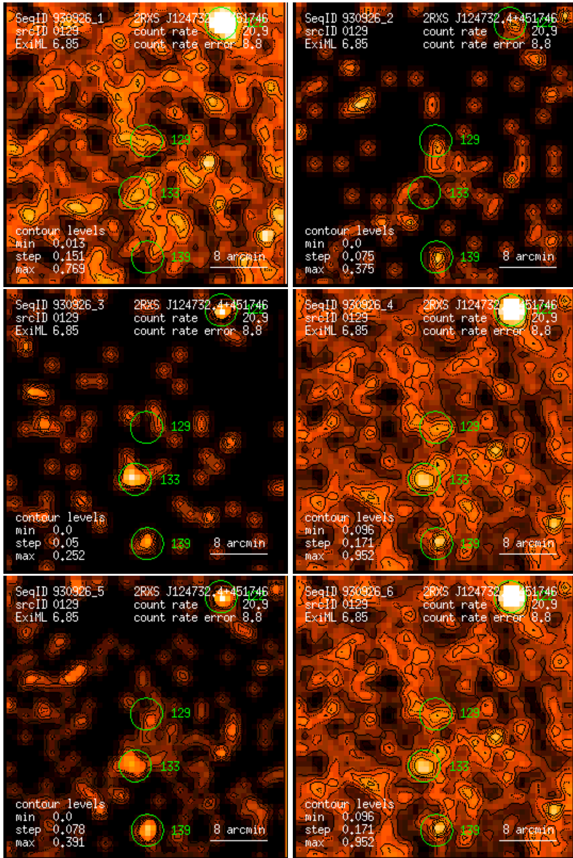
Figure 129: RASS 930926: detection 0129: band rate images, Gaussian filter: (1) PSPC channels 11 – 41, (2) 52 – 90, (3) 91 – 201, (4) 11 – 235, (5) 52 – 201, (6) 11 – 201. Broad band rates in counts/ks. Band rate contour levels in counts/ks/arcmin 2 .
