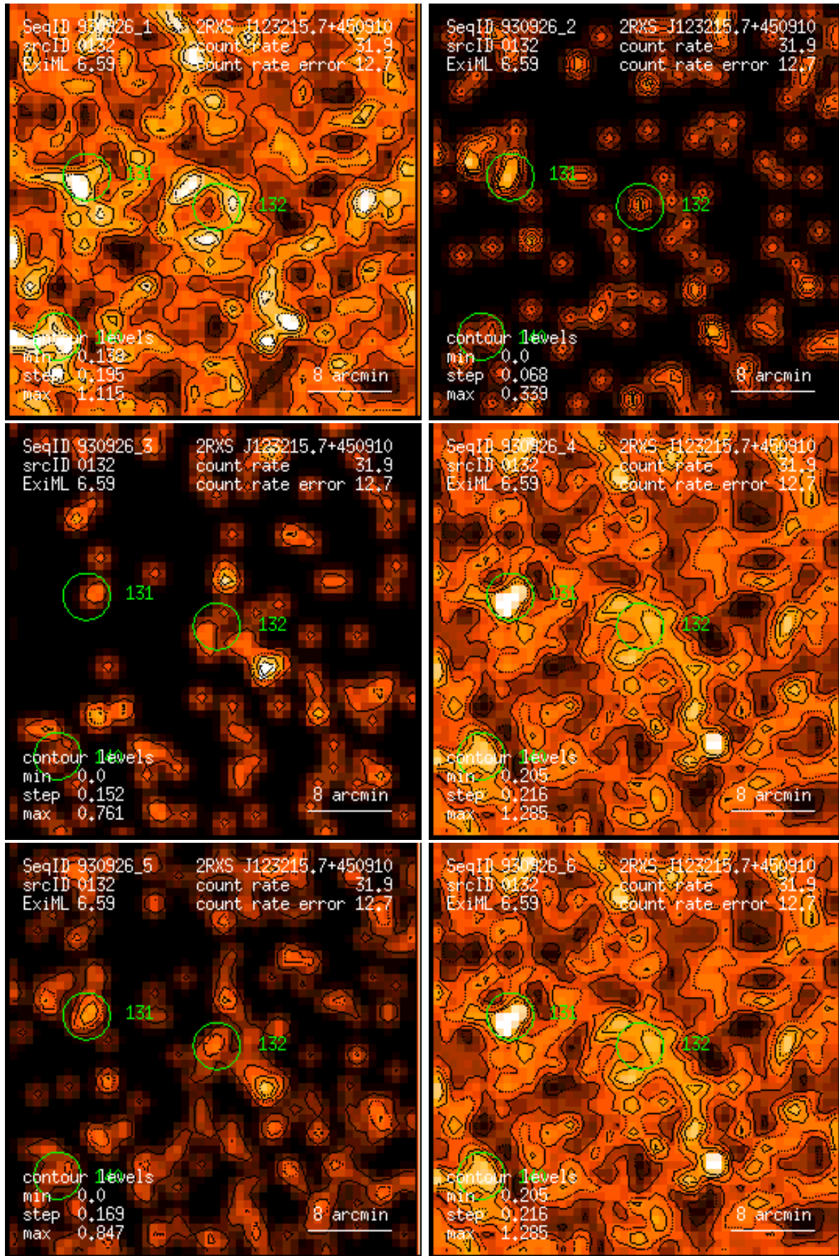
Figure 132: RASS 930926: detection 0132: band rate images, Gaussian filter: (1) PSPC channels 11 – 41, (2) 52 – 90, (3) 91 – 201, (4) 11 – 235, (5) 52 – 201, (6) 11 – 201. Broad band rates in counts/ks. Band rate contour levels in counts/ks/arcmin 2 .
