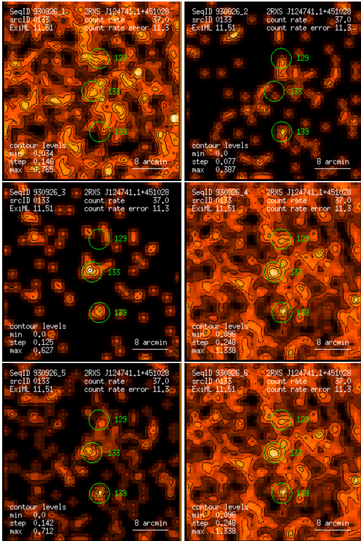
Figure 133: RASS 930926: detection 0133: band rate images, Gaussian filter: (1) PSPC channels 11 – 41, (2) 52 – 90, (3) 91 – 201, (4) 11 – 235, (5) 52 – 201, (6) 11 – 201. Broad band rates in counts/ks. Band rate contour levels in counts/ks/arcmin 2 .
