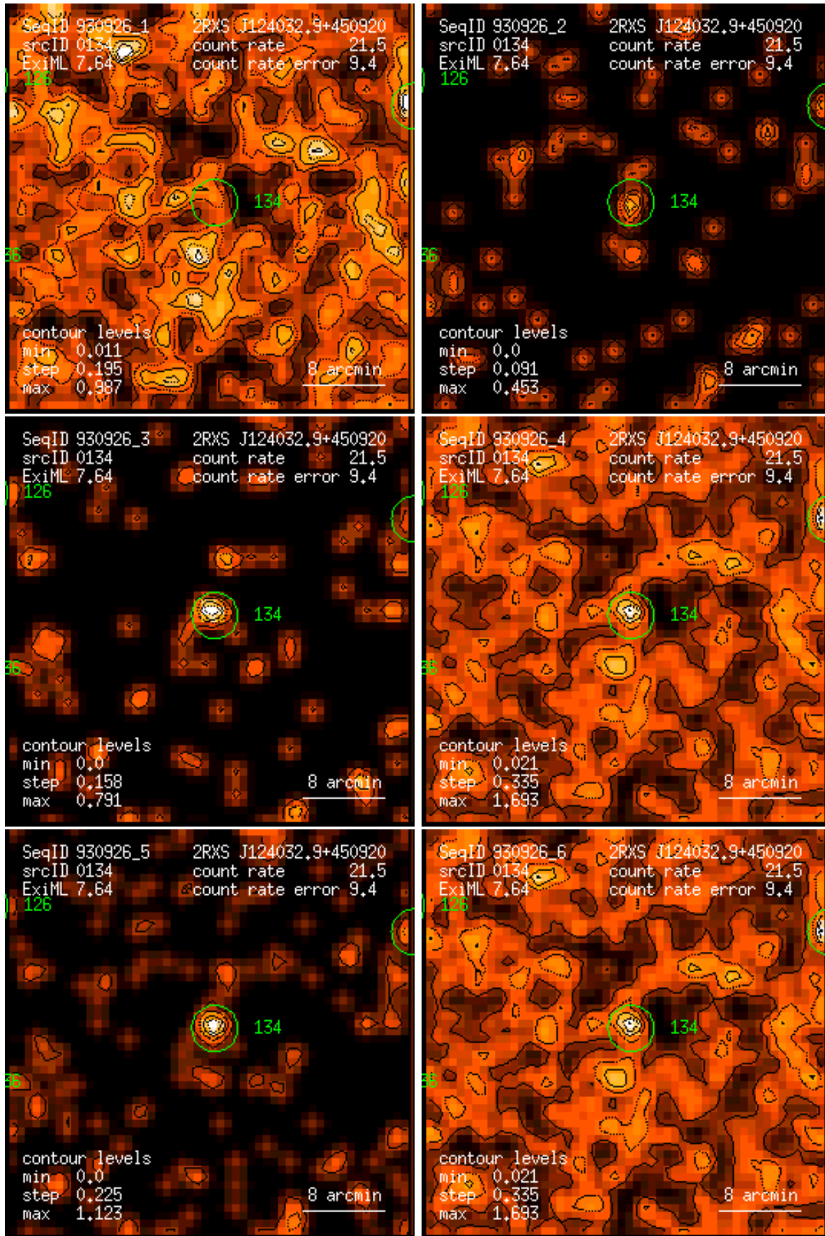
Figure 134: RASS 930926: detection 0134: band rate images, Gaussian filter: (1) PSPC channels 11 – 41, (2) 52 – 90, (3) 91 – 201, (4) 11 – 235, (5) 52 – 201, (6) 11 – 201. Broad band rates in counts/ks. Band rate contour levels in counts/ks/arcmin 2 .
