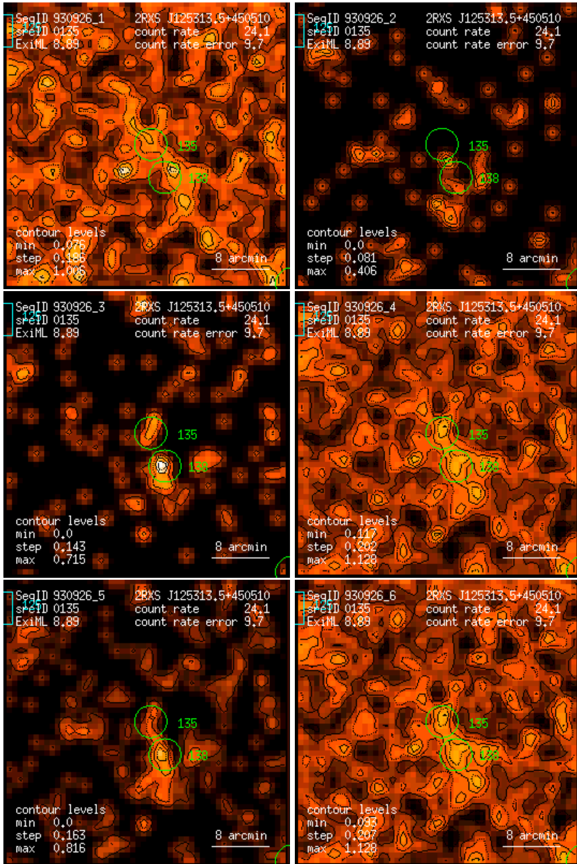
Figure 135: RASS 930926: detection 0135: band rate images, Gaussian filter: (1) PSPC channels 11 – 41, (2) 52 – 90, (3) 91 – 201, (4) 11 – 235, (5) 52 – 201, (6) 11 – 201. Broad band rates in counts/ks. Band rate contour levels in counts/ks/arcmin 2 .
