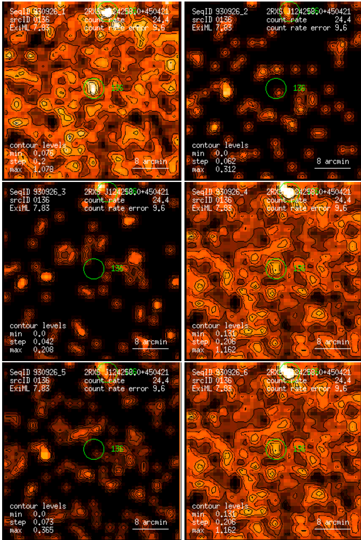
Figure 136: RASS 930926: detection 0136: band rate images, Gaussian filter: (1) PSPC channels 11 – 41, (2) 52 – 90, (3) 91 – 201, (4) 11 – 235, (5) 52 – 201, (6) 11 – 201. Broad band rates in counts/ks. Band rate contour levels in counts/ks/arcmin 2 .
