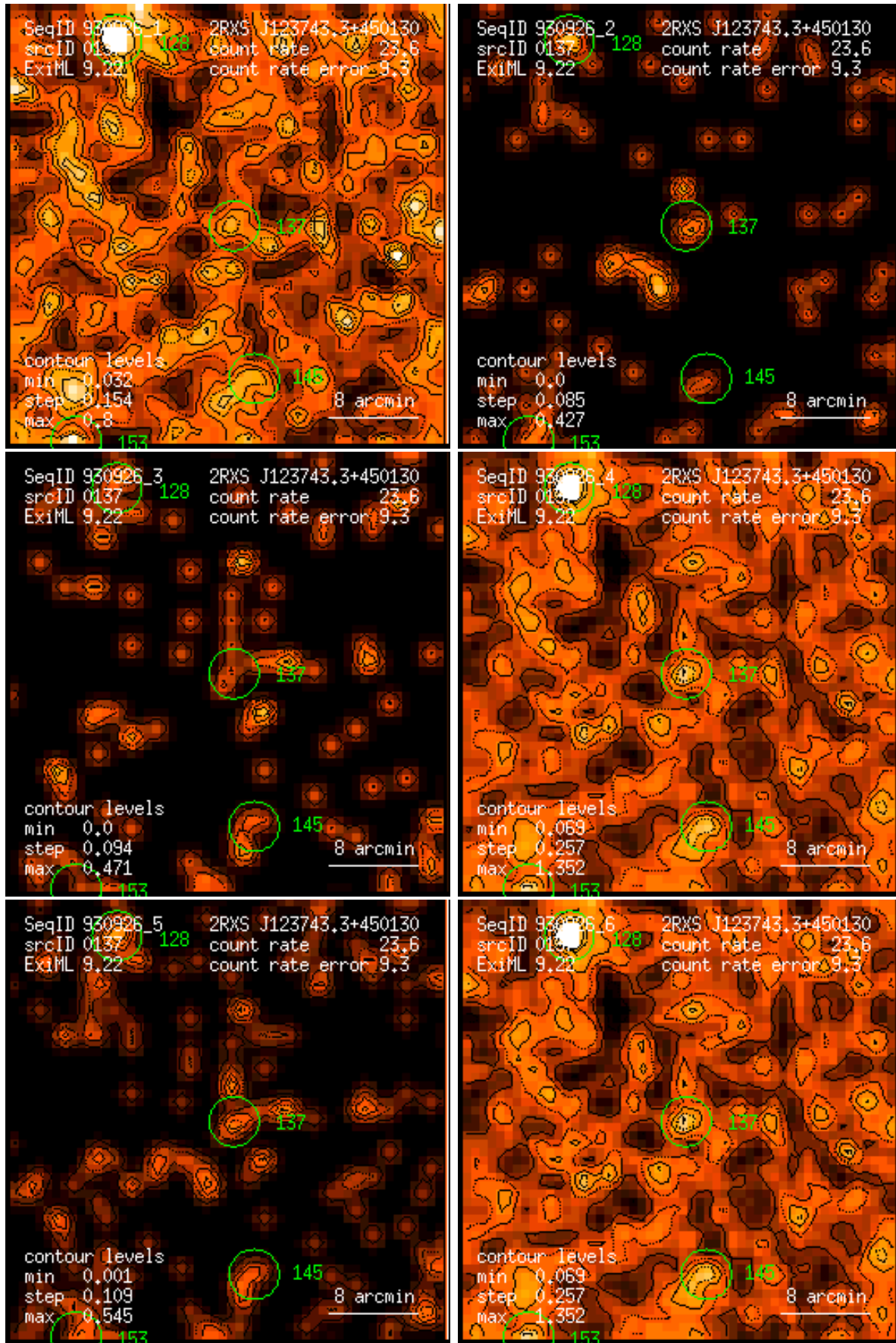
Figure 137: RASS 930926: detection 0137: band rate images, Gaussian filter: (1) PSPC channels 11 – 41, (2) 52 – 90, (3) 91 – 201, (4) 11 – 235, (5) 52 – 201, (6) 11 – 201. Broad band rates in counts/ks. Band rate contour levels in counts/ks/arcmin 2 .
