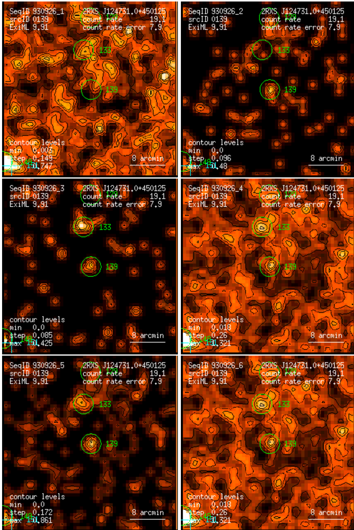
Figure 139: RASS 930926: detection 0139: band rate images, Gaussian filter: (1) PSPC channels 11 – 41, (2) 52 – 90, (3) 91 – 201, (4) 11 – 235, (5) 52 – 201, (6) 11 – 201. Broad band rates in counts/ks. Band rate contour levels in counts/ks/arcmin 2 .
