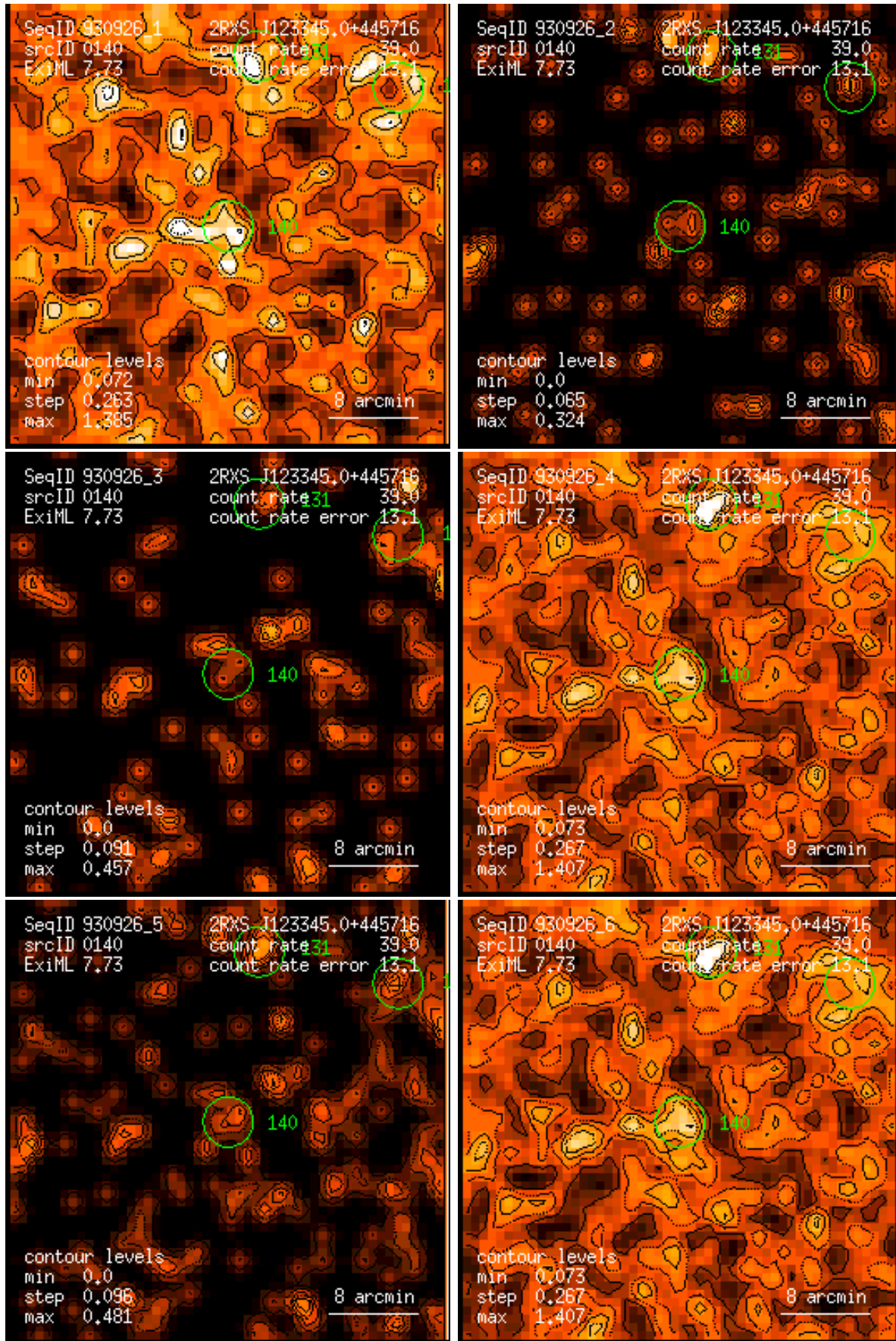
Figure 140: RASS 930926: detection 0140: band rate images, Gaussian filter: (1) PSPC channels 11 – 41, (2) 52 – 90, (3) 91 – 201, (4) 11 – 235, (5) 52 – 201, (6) 11 – 201. Broad band rates in counts/ks. Band rate contour levels in counts/ks/arcmin 2 .
