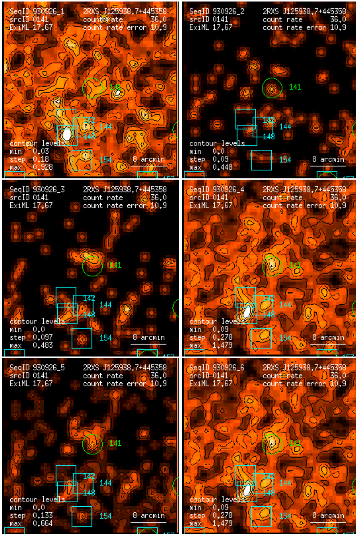
Figure 141: RASS 930926: detection 0141: band rate images, Gaussian filter: (1) PSPC channels 11 – 41, (2) 52 – 90, (3) 91 – 201, (4) 11 – 235, (5) 52 – 201, (6) 11 – 201. Broad band rates in counts/ks. Band rate contour levels in counts/ks/arcmin 2 .
