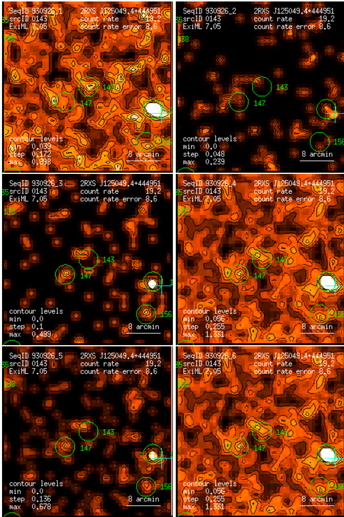
Figure 143: RASS 930926: detection 0143: band rate images, Gaussian filter: (1) PSPC channels 11 – 41, (2) 52 – 90, (3) 91 – 201, (4) 11 – 235, (5) 52 – 201, (6) 11 – 201. Broad band rates in counts/ks. Band rate contour levels in counts/ks/arcmin 2 .
