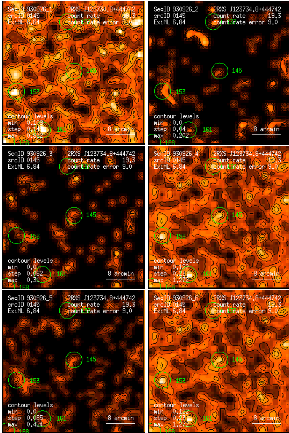
Figure 145: RASS 930926: detection 0145: band rate images, Gaussian filter: (1) PSPC channels 11 – 41, (2) 52 – 90, (3) 91 – 201, (4) 11 – 235, (5) 52 – 201, (6) 11 – 201. Broad band rates in counts/ks. Band rate contour levels in counts/ks/arcmin 2 .
