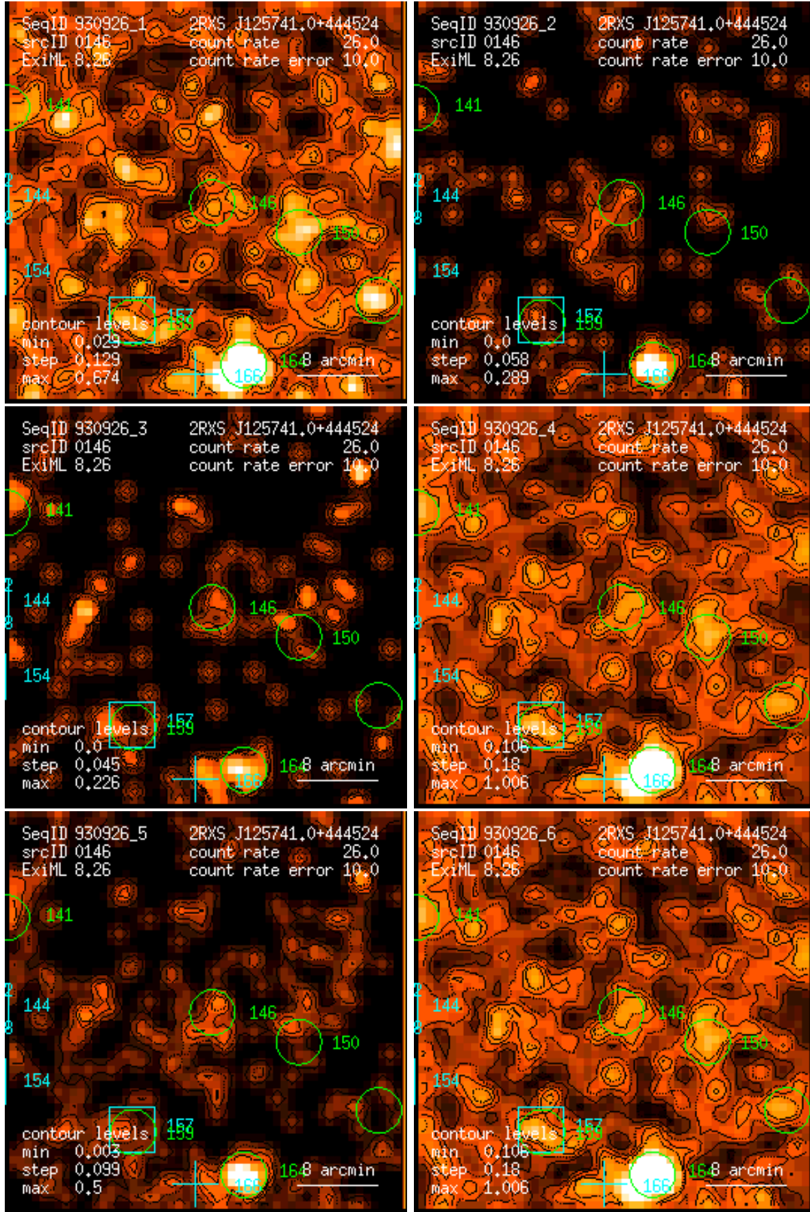
Figure 146: RASS 930926: detection 0146: band rate images, Gaussian filter: (1) PSPC channels 11 – 41, (2) 52 – 90, (3) 91 – 201, (4) 11 – 235, (5) 52 – 201, (6) 11 – 201. Broad band rates in counts/ks. Band rate contour levels in counts/ks/arcmin 2 .
