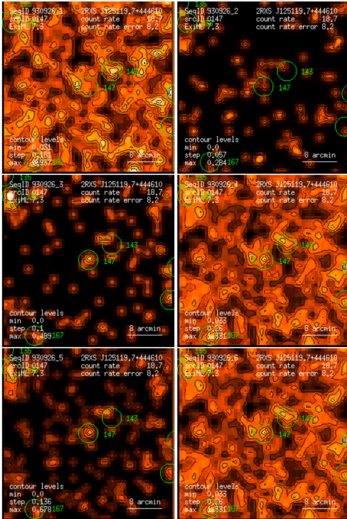
Figure 147: RASS 930926: detection 0147: band rate images, Gaussian filter: (1) PSPC channels 11 – 41, (2) 52 – 90, (3) 91 – 201, (4) 11 – 235, (5) 52 – 201, (6) 11 – 201. Broad band rates in counts/ks. Band rate contour levels in counts/ks/arcmin 2 .
