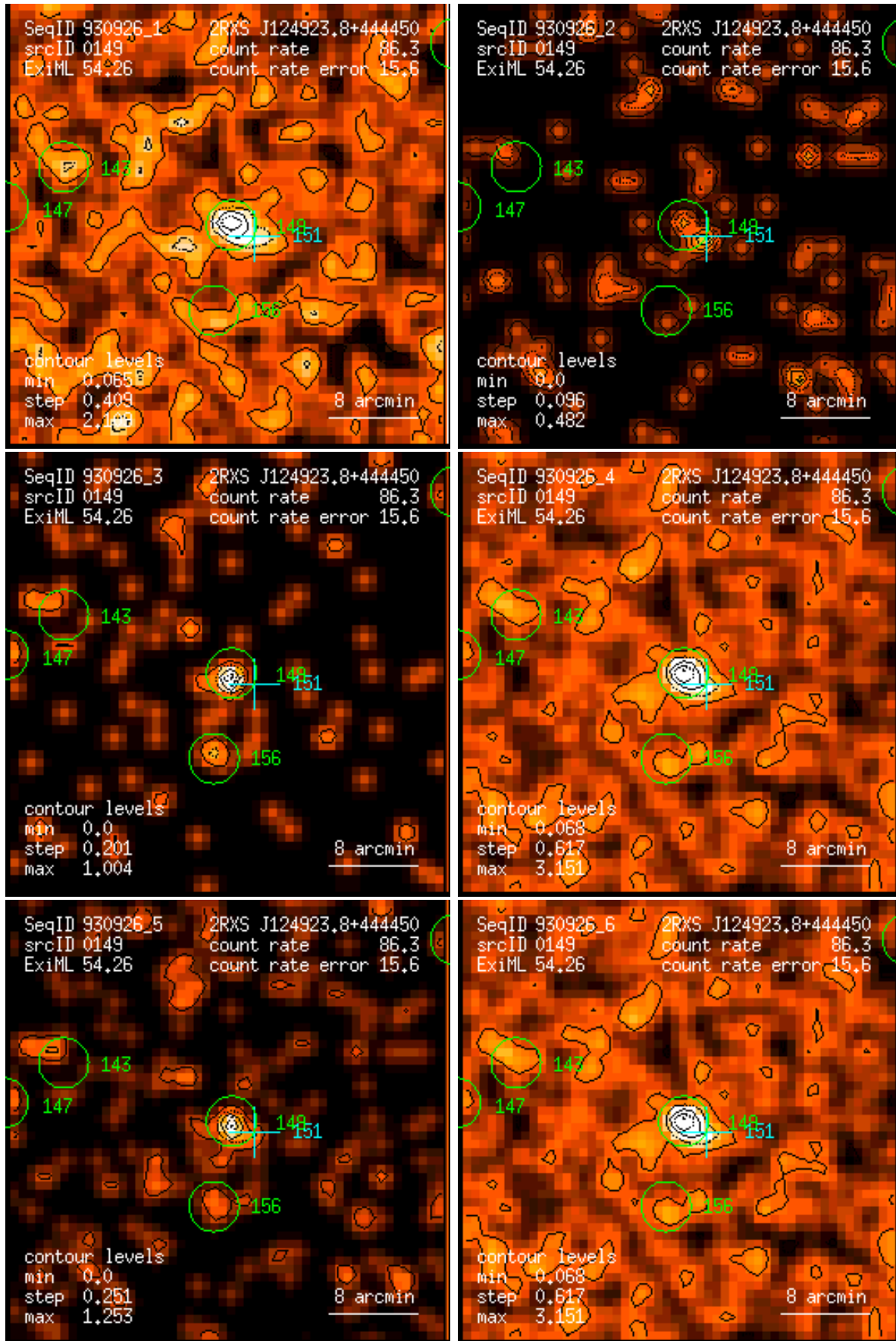
Figure 149: RASS 930926: detection 0149: band rate images, Gaussian filter: (1) PSPC channels 11 – 41, (2) 52 – 90, (3) 91 – 201, (4) 11 – 235, (5) 52 – 201, (6) 11 – 201. Broad band rates in counts/ks. Band rate contour levels in counts/ks/arcmin 2 .
