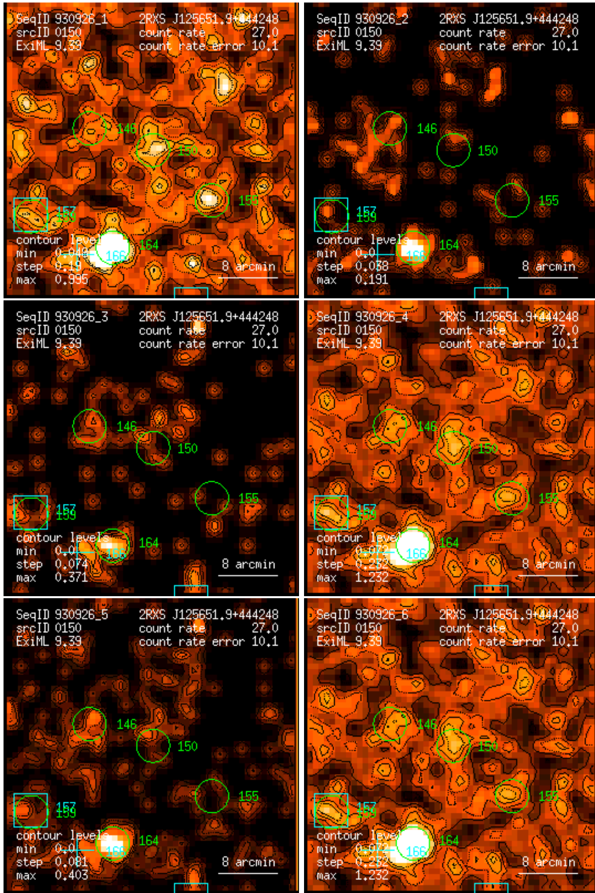
Figure 150: RASS 930926: detection 0150: band rate images, Gaussian filter: (1) PSPC channels 11 – 41, (2) 52 – 90, (3) 91 – 201, (4) 11 – 235, (5) 52 – 201, (6) 11 – 201. Broad band rates in counts/ks. Band rate contour levels in counts/ks/arcmin 2 .
