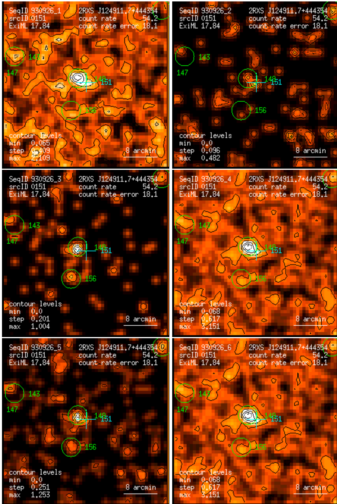
Figure 151: RASS 930926: detection 0151: band rate images, Gaussian filter: (1) PSPC channels 11 – 41, (2) 52 – 90, (3) 91 – 201, (4) 11 – 235, (5) 52 – 201, (6) 11 – 201. Broad band rates in counts/ks. Band rate contour levels in counts/ks/arcmin 2 .
