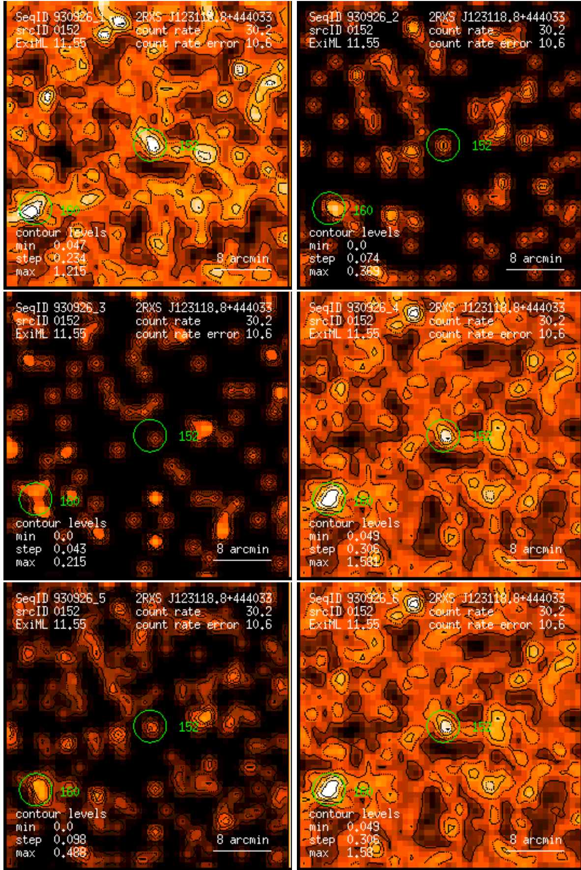
Figure 152: RASS 930926: detection 0152: band rate images, Gaussian filter: (1) PSPC channels 11 – 41, (2) 52 – 90, (3) 91 – 201, (4) 11 – 235, (5) 52 – 201, (6) 11 – 201. Broad band rates in counts/ks. Band rate contour levels in counts/ks/arcmin 2 .
