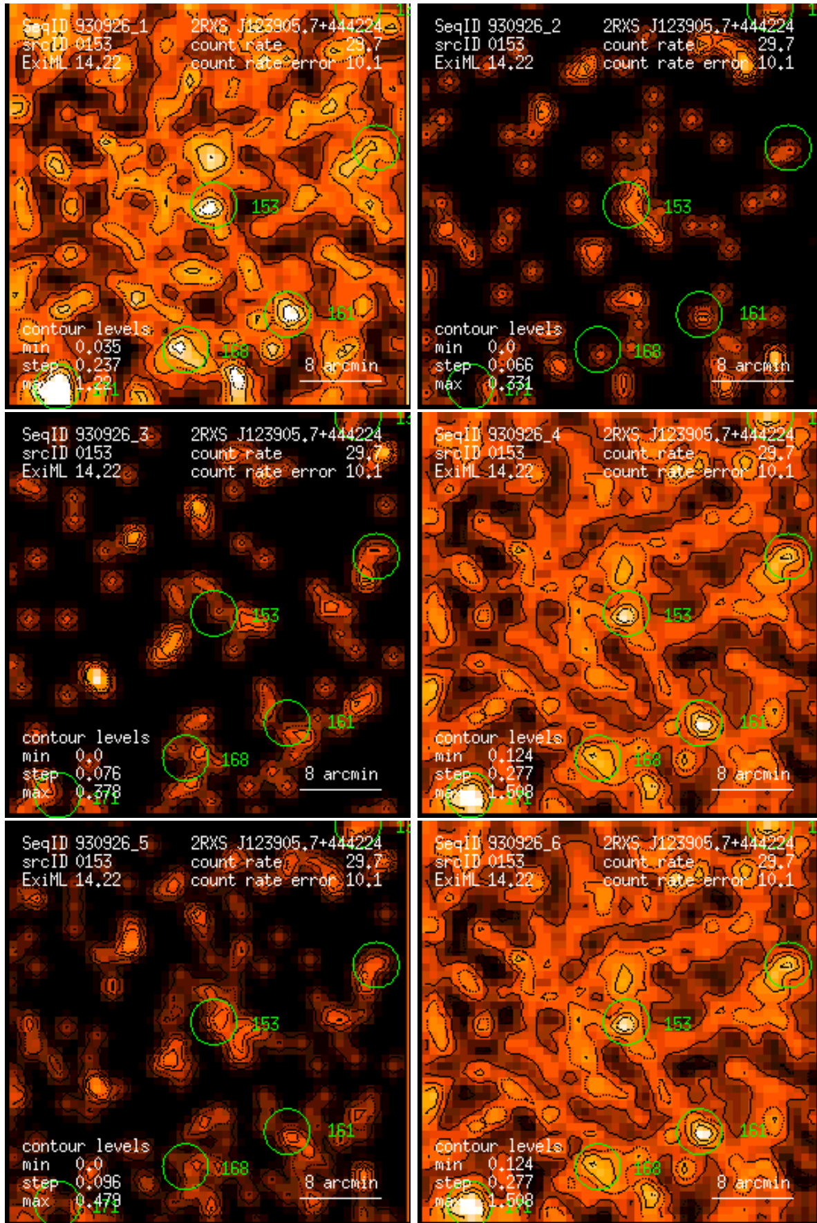
Figure 153: RASS 930926: detection 0153: band rate images, Gaussian filter: (1) PSPC channels 11 – 41, (2) 52 – 90, (3) 91 – 201, (4) 11 – 235, (5) 52 – 201, (6) 11 – 201. Broad band rates in counts/ks. Band rate contour levels in counts/ks/arcmin 2 .
