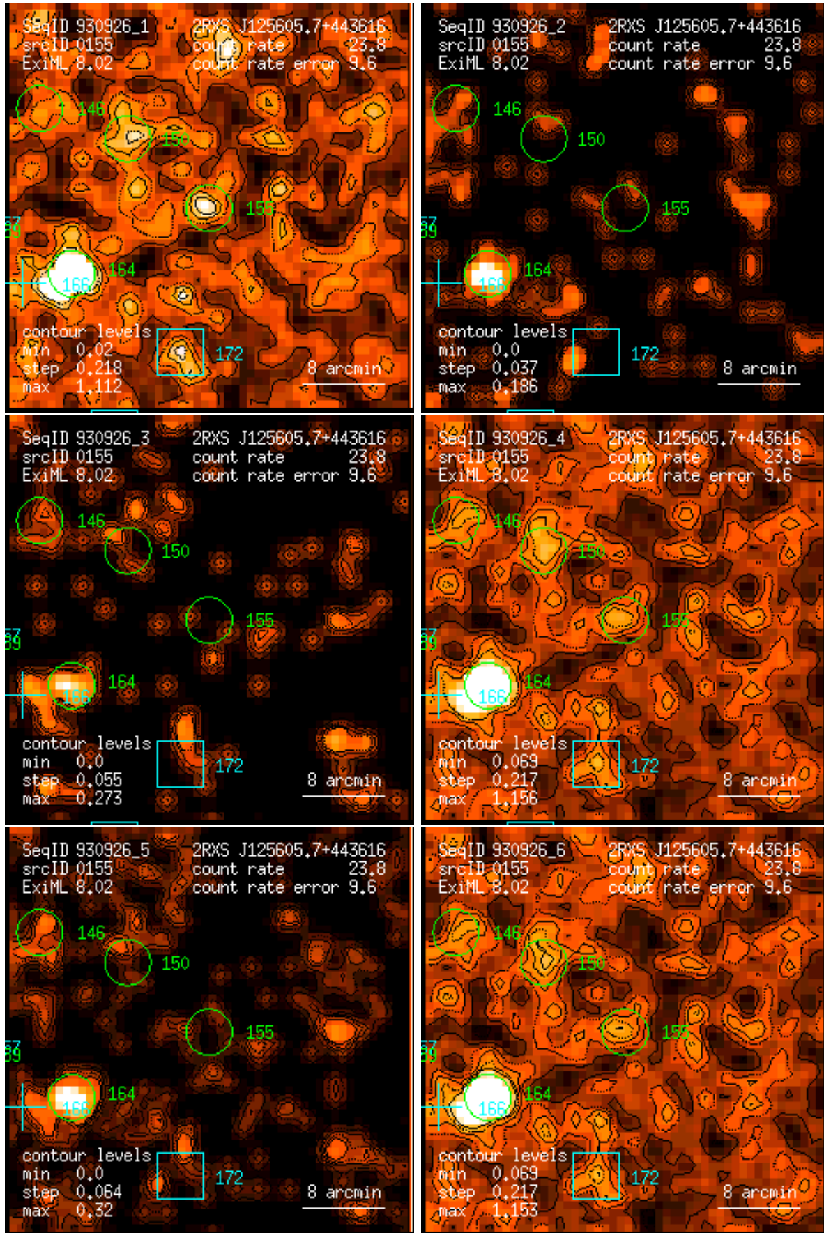
Figure 155: RASS 930926: detection 0155: band rate images, Gaussian filter: (1) PSPC channels 11 – 41, (2) 52 – 90, (3) 91 – 201, (4) 11 – 235, (5) 52 – 201, (6) 11 – 201. Broad band rates in counts/ks. Band rate contour levels in counts/ks/arcmin 2 .
