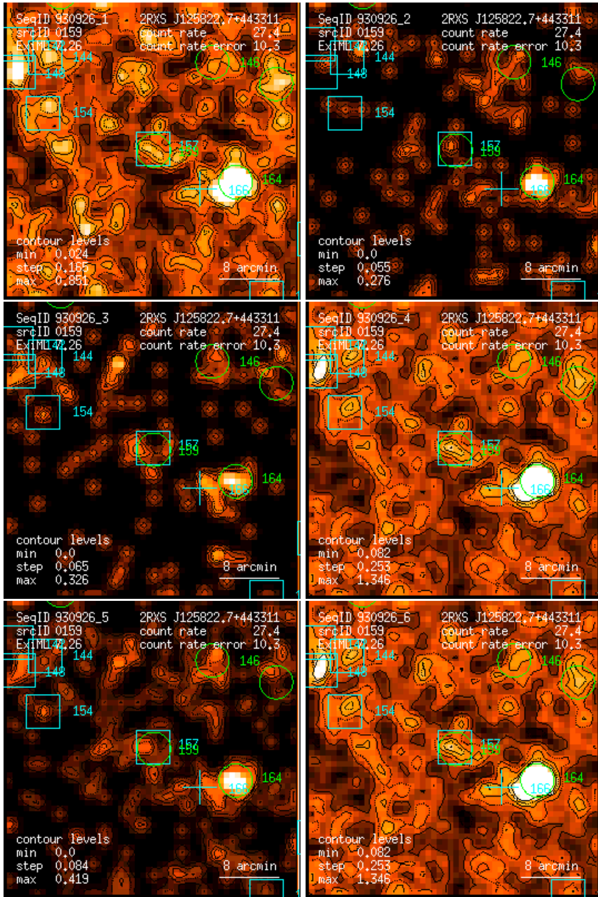
Figure 159: RASS 930926: detection 0159: band rate images, Gaussian filter: (1) PSPC channels 11 – 41, (2) 52 – 90, (3) 91 – 201, (4) 11 – 235, (5) 52 – 201, (6) 11 – 201. Broad band rates in counts/ks. Band rate contour levels in counts/ks/arcmin 2 .
