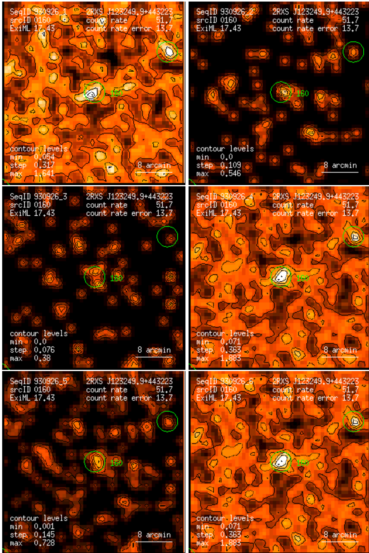
Figure 160: RASS 930926: detection 0160: band rate images, Gaussian filter: (1) PSPC channels 11 – 41, (2) 52 – 90, (3) 91 – 201, (4) 11 – 235, (5) 52 – 201, (6) 11 – 201. Broad band rates in counts/ks. Band rate contour levels in counts/ks/arcmin 2 .
