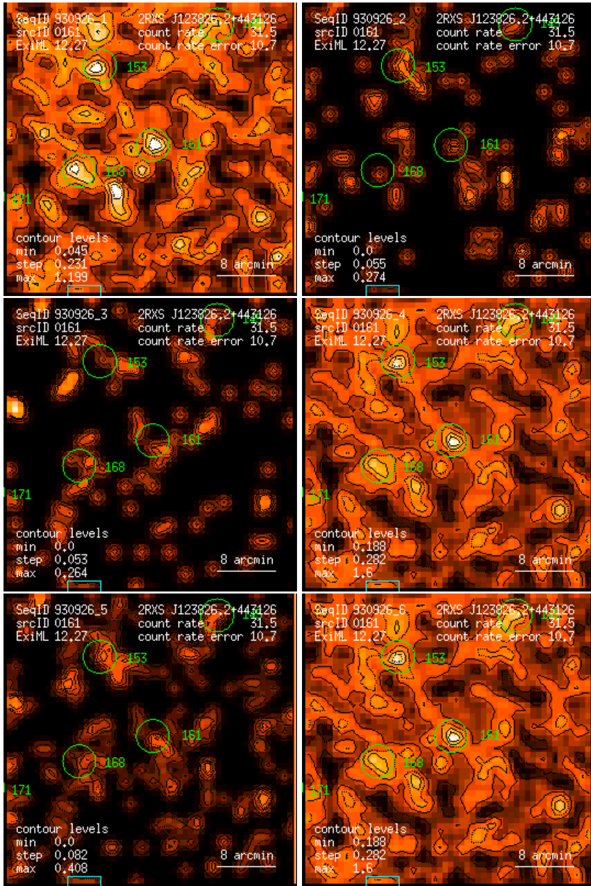
Figure 161: RASS 930926: detection 0161: band rate images, Gaussian filter: (1) PSPC channels 11 – 41, (2) 52 – 90, (3) 91 – 201, (4) 11 – 235, (5) 52 – 201, (6) 11 – 201. Broad band rates in counts/ks. Band rate contour levels in counts/ks/arcmin 2 .
