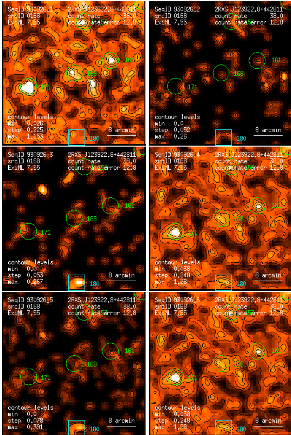
Figure 168: RASS 930926: detection 0168: band rate images, Gaussian filter: (1) PSPC channels 11 – 41, (2) 52 – 90, (3) 91 – 201, (4) 11 – 235, (5) 52 – 201, (6) 11 – 201. Broad band rates in counts/ks. Band rate contour levels in counts/ks/arcmin 2 .
