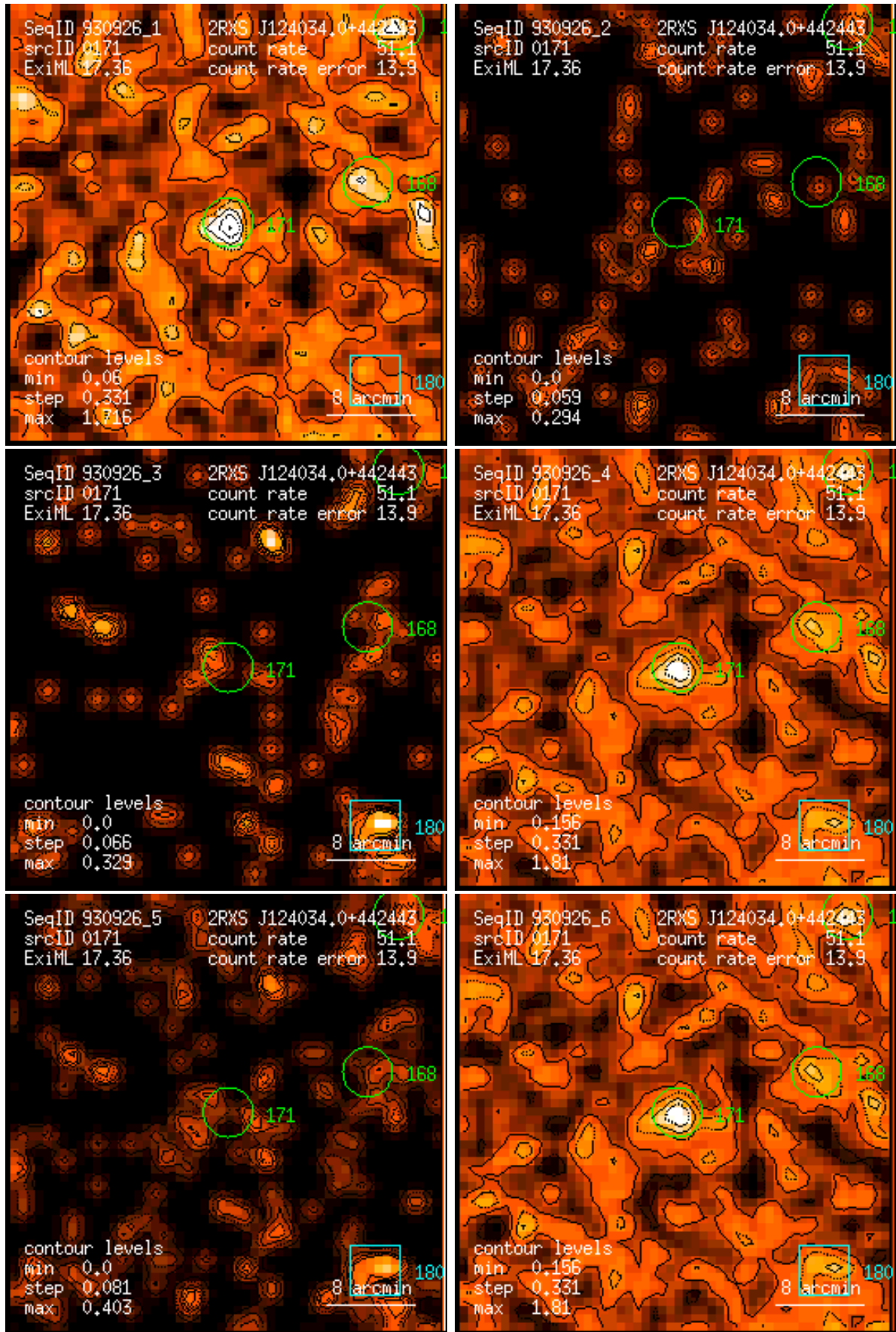
Figure 171: RASS 930926: detection 0171: band rate images, Gaussian filter: (1) PSPC channels 11 – 41, (2) 52 – 90, (3) 91 – 201, (4) 11 – 235, (5) 52 – 201, (6) 11 – 201. Broad band rates in counts/ks. Band rate contour levels in counts/ks/arcmin 2 .
