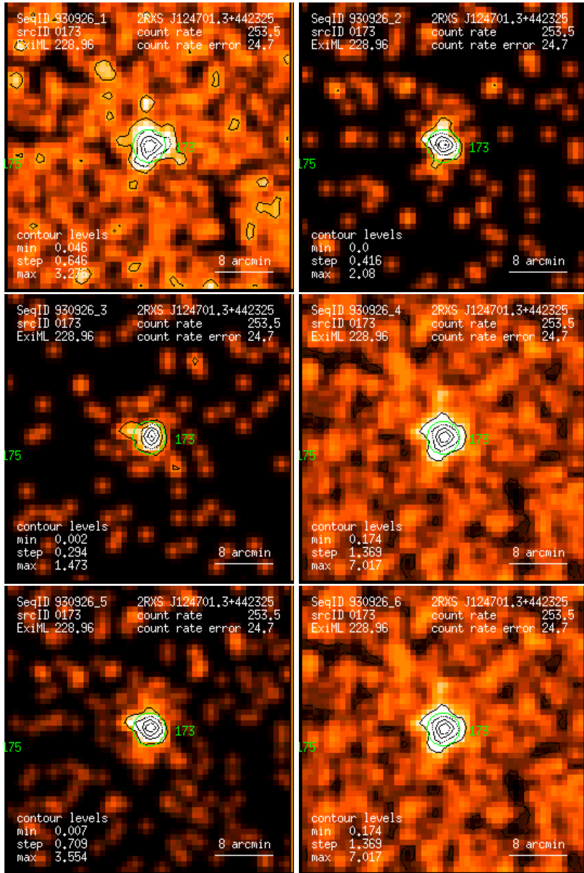
Figure 173: RASS 930926: detection 0173: band rate images, Gaussian filter: (1) PSPC channels 11 – 41, (2) 52 – 90, (3) 91 – 201, (4) 11 – 235, (5) 52 – 201, (6) 11 – 201. Broad band rates in counts/ks. Band rate contour levels in counts/ks/arcmin 2 .
