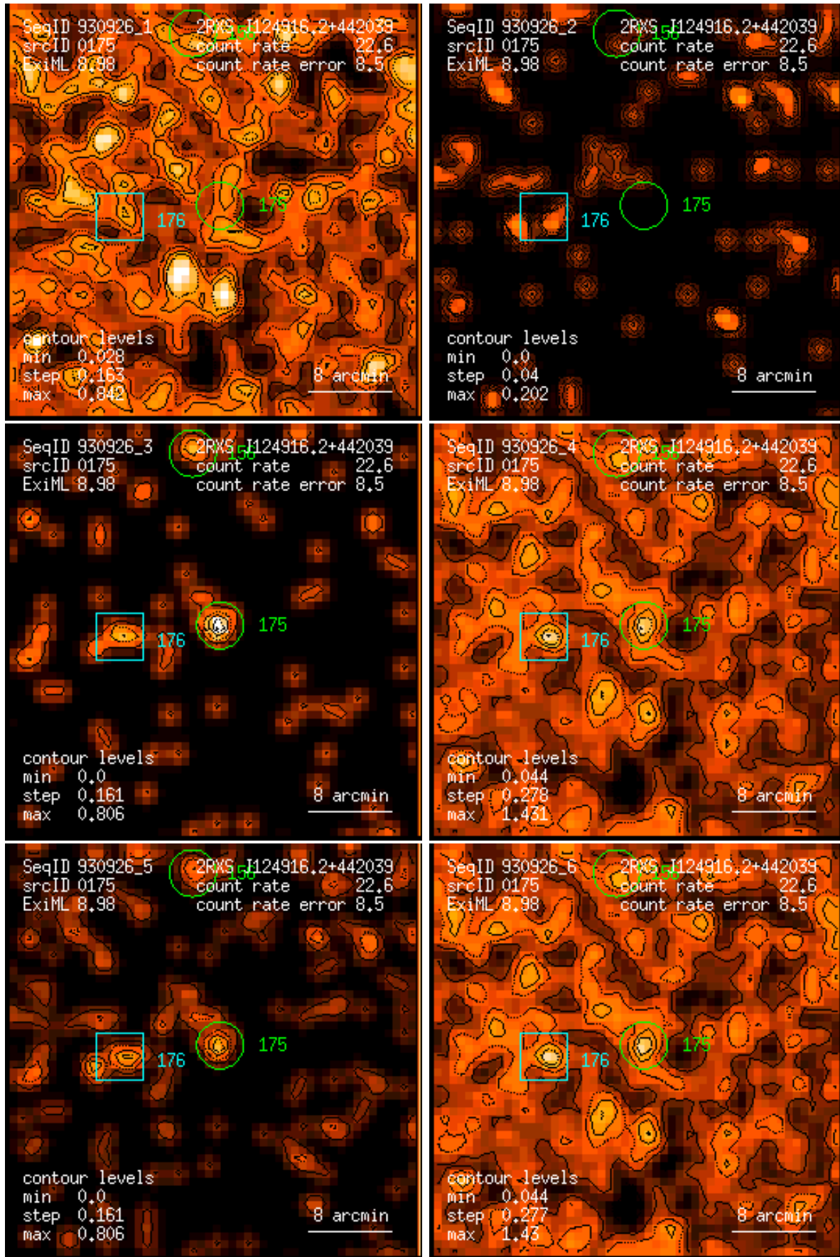
Figure 175: RASS 930926: detection 0175: band rate images, Gaussian filter: (1) PSPC channels 11 – 41, (2) 52 – 90, (3) 91 – 201, (4) 11 – 235, (5) 52 – 201, (6) 11 – 201. Broad band rates in counts/ks. Band rate contour levels in counts/ks/arcmin 2 .
