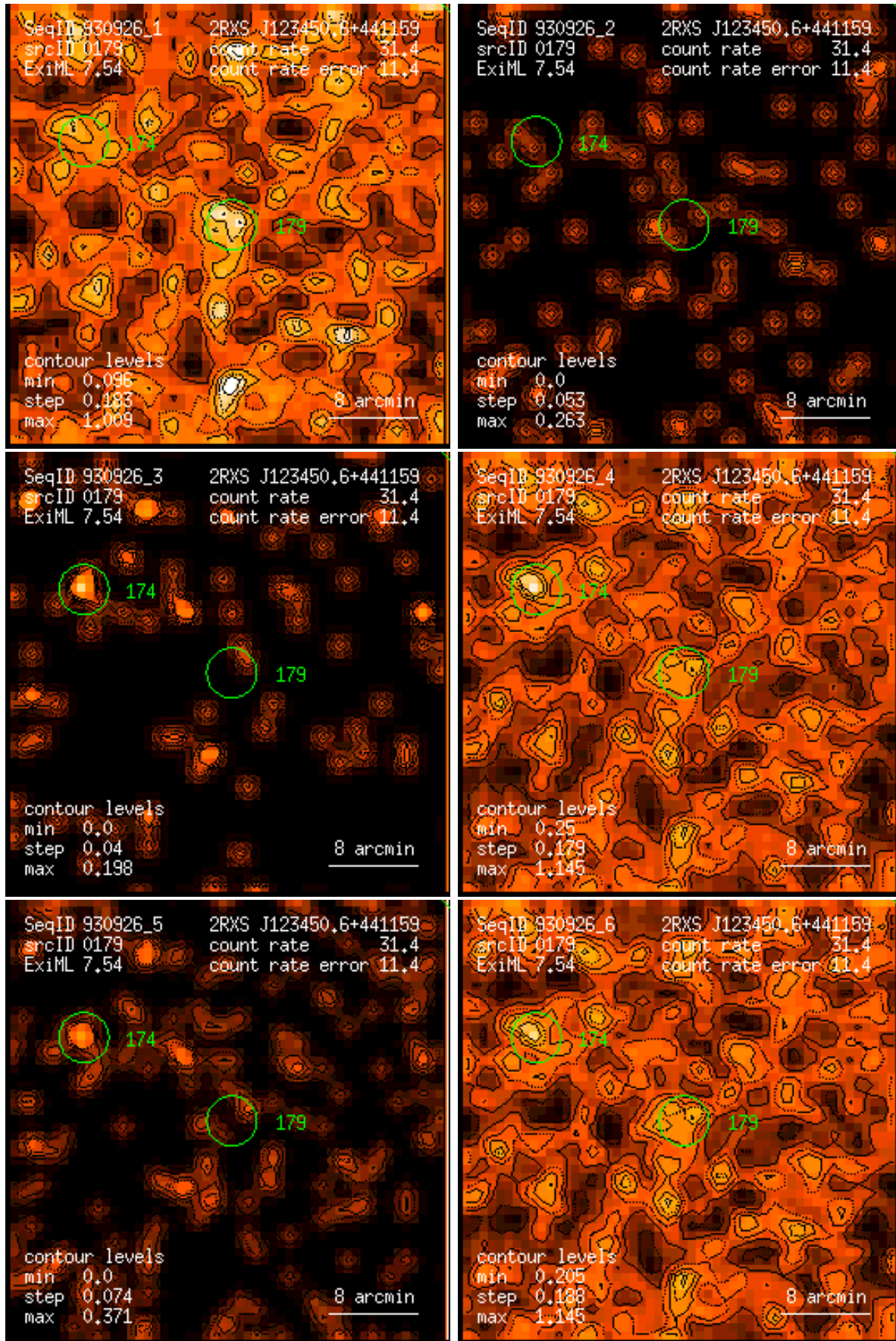
Figure 179: RASS 930926: detection 0179: band rate images, Gaussian filter: (1) PSPC channels 11 – 41, (2) 52 – 90, (3) 91 – 201, (4) 11 – 235, (5) 52 – 201, (6) 11 – 201. Broad band rates in counts/ks. Band rate contour levels in counts/ks/arcmin 2 .
