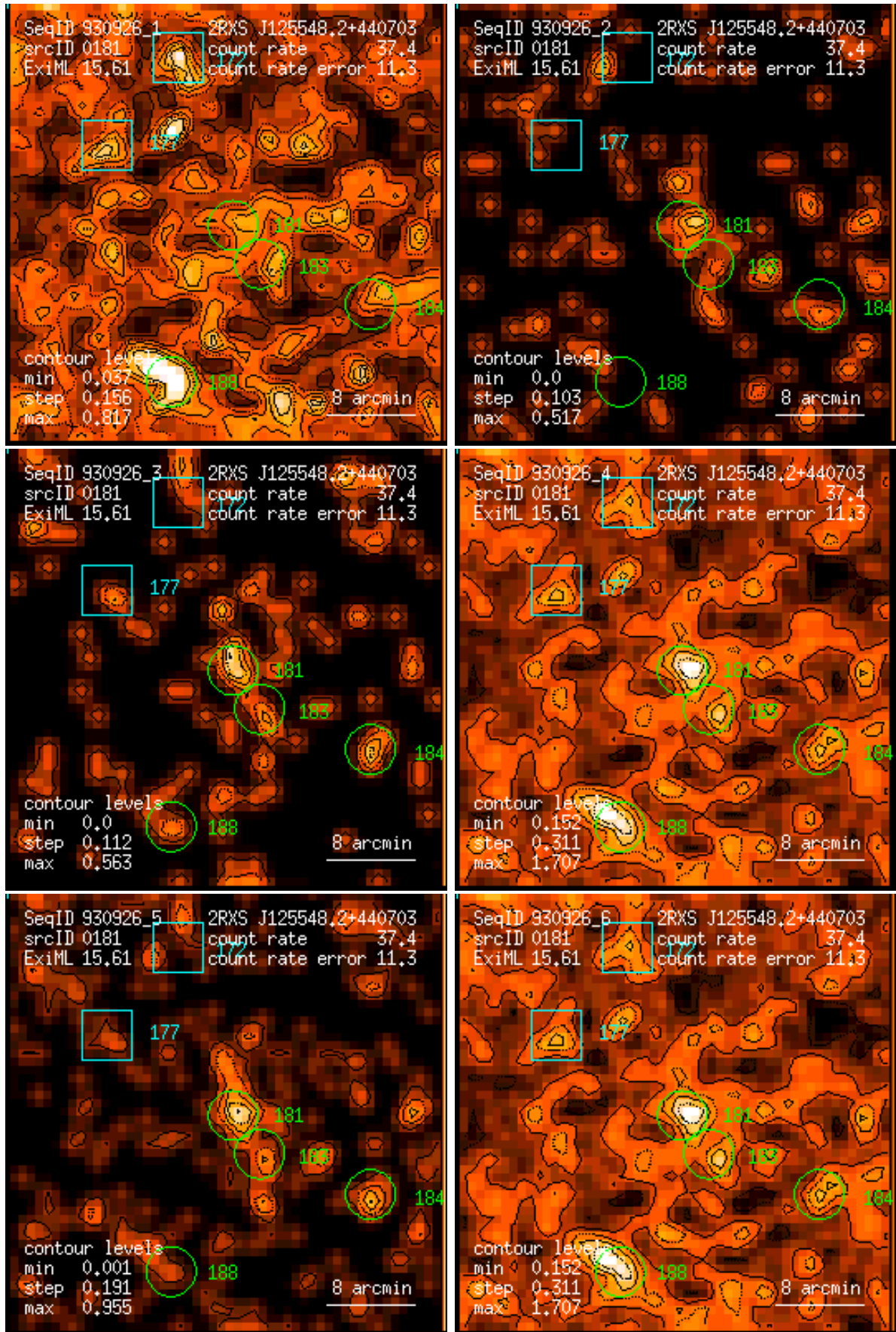
Figure 181: RASS 930926: detection 0181: band rate images, Gaussian filter: (1) PSPC channels 11 – 41, (2) 52 – 90, (3) 91 – 201, (4) 11 – 235, (5) 52 – 201, (6) 11 – 201. Broad band rates in counts/ks. Band rate contour levels in counts/ks/arcmin 2 .
