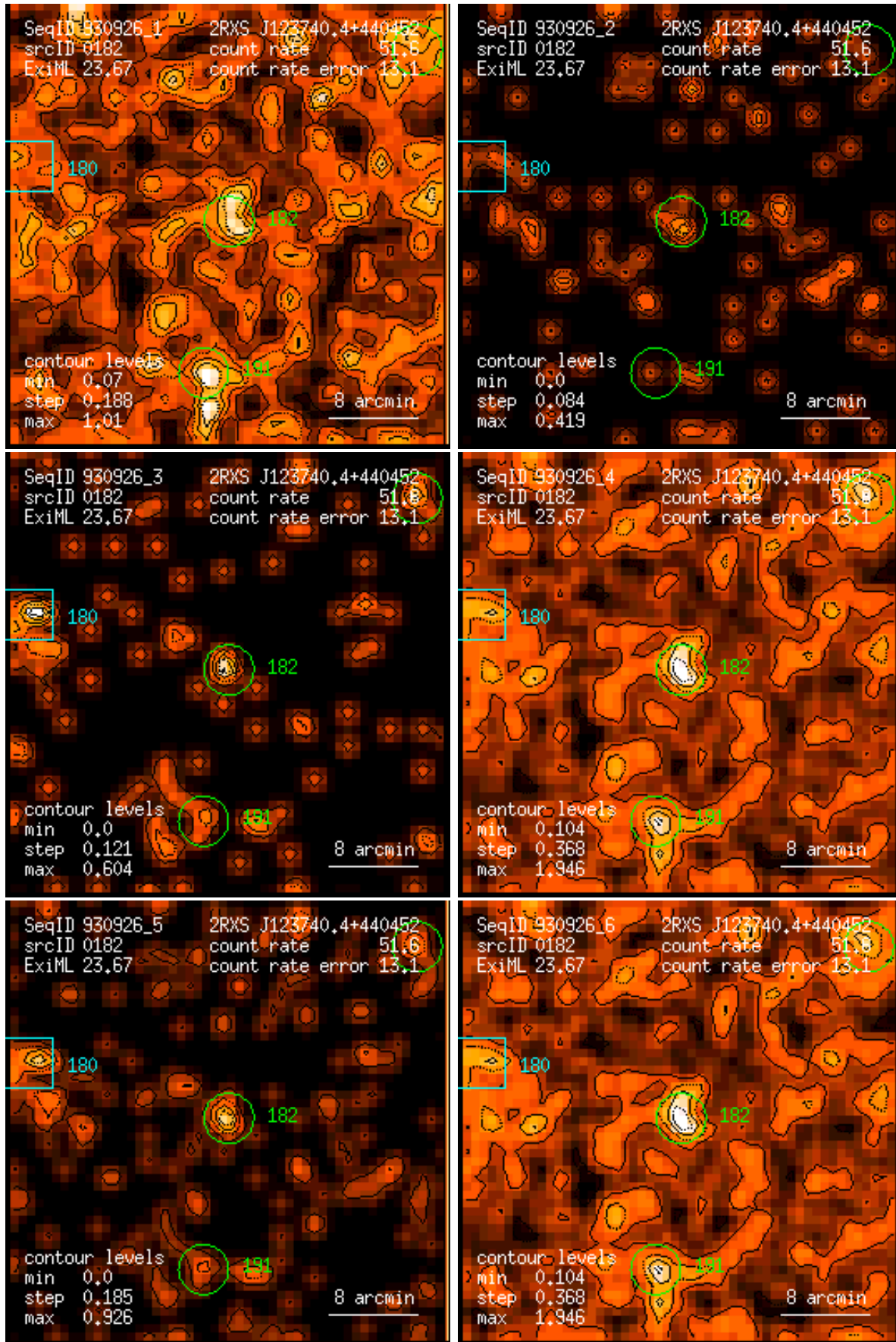
Figure 182: RASS 930926: detection 0182: band rate images, Gaussian filter: (1) PSPC channels 11 – 41, (2) 52 – 90, (3) 91 – 201, (4) 11 – 235, (5) 52 – 201, (6) 11 – 201. Broad band rates in counts/ks. Band rate contour levels in counts/ks/arcmin 2 .
