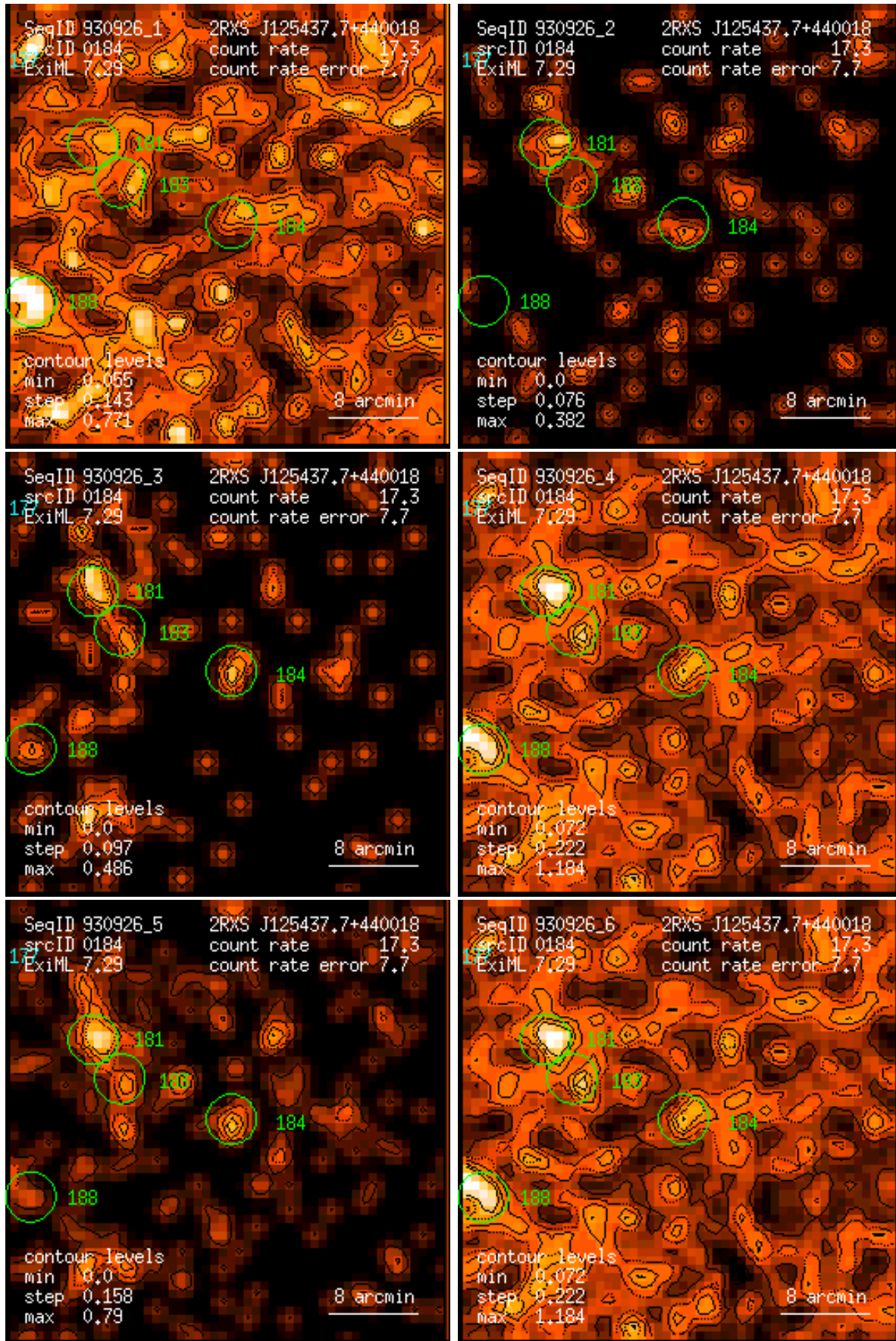
Figure 184: RASS 930926: detection 0184: band rate images, Gaussian filter: (1) PSPC channels 11 – 41, (2) 52 – 90, (3) 91 – 201, (4) 11 – 235, (5) 52 – 201, (6) 11 – 201. Broad band rates in counts/ks. Band rate contour levels in counts/ks/arcmin 2 .
