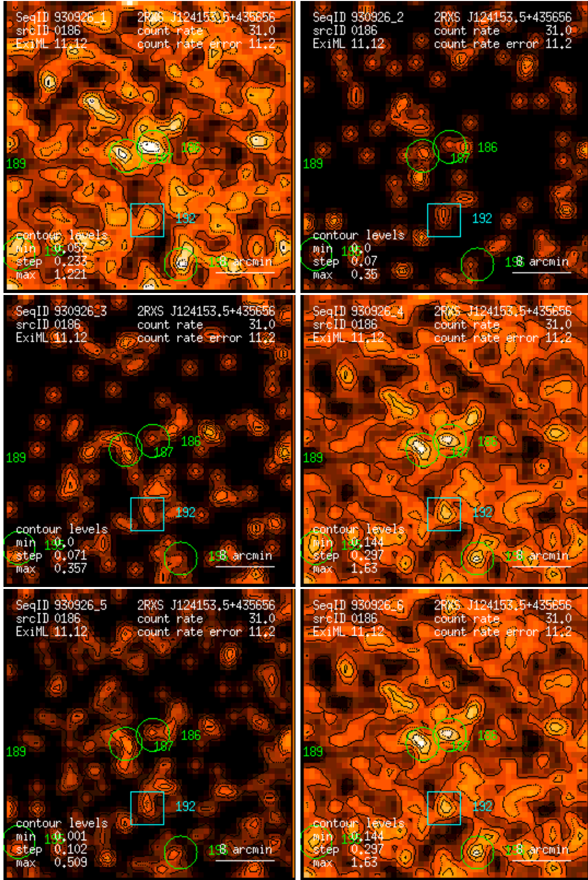
Figure 186: RASS 930926: detection 0186: band rate images, Gaussian filter: (1) PSPC channels 11 – 41, (2) 52 – 90, (3) 91 – 201, (4) 11 – 235, (5) 52 – 201, (6) 11 – 201. Broad band rates in counts/ks. Band rate contour levels in counts/ks/arcmin 2 .
