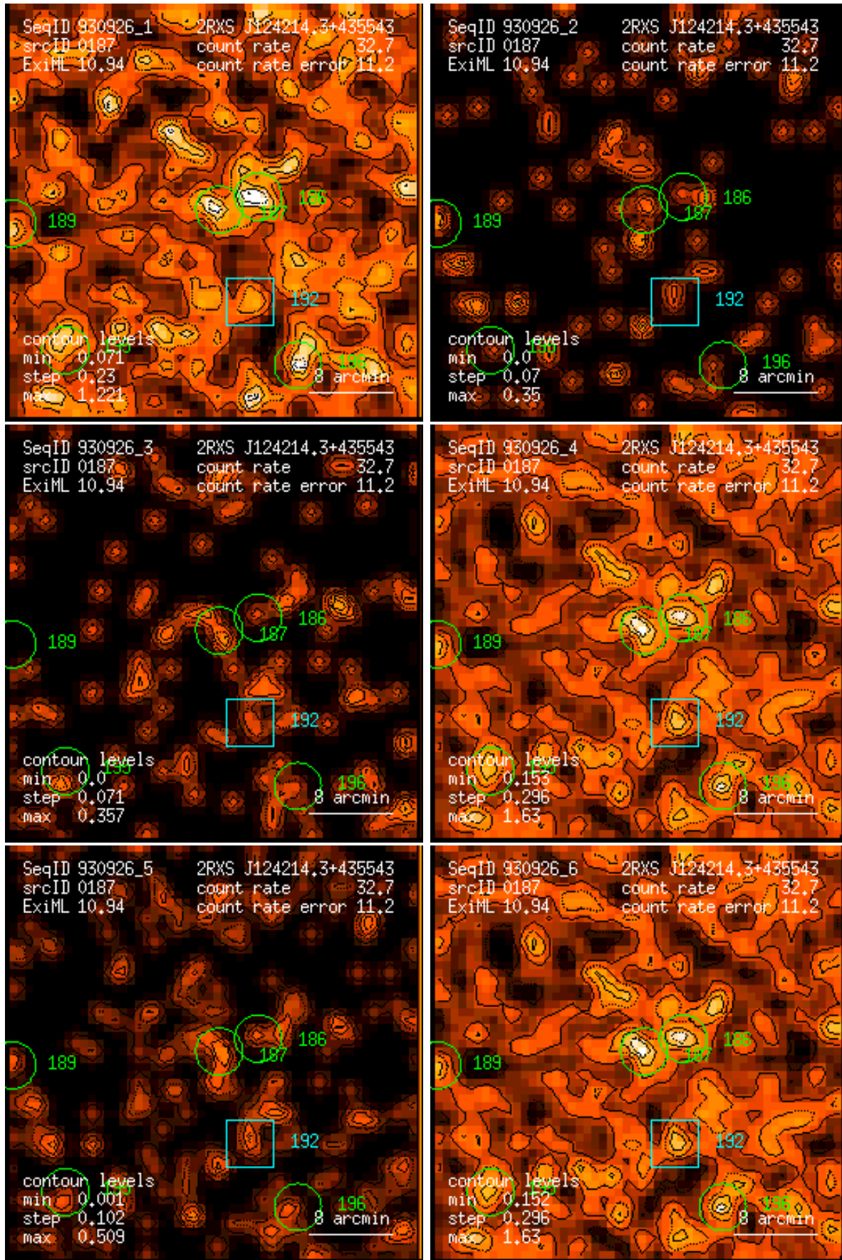
Figure 187: RASS 930926: detection 0187: band rate images, Gaussian filter: (1) PSPC channels 11 – 41, (2) 52 – 90, (3) 91 – 201, (4) 11 – 235, (5) 52 – 201, (6) 11 – 201. Broad band rates in counts/ks. Band rate contour levels in counts/ks/arcmin 2 .
