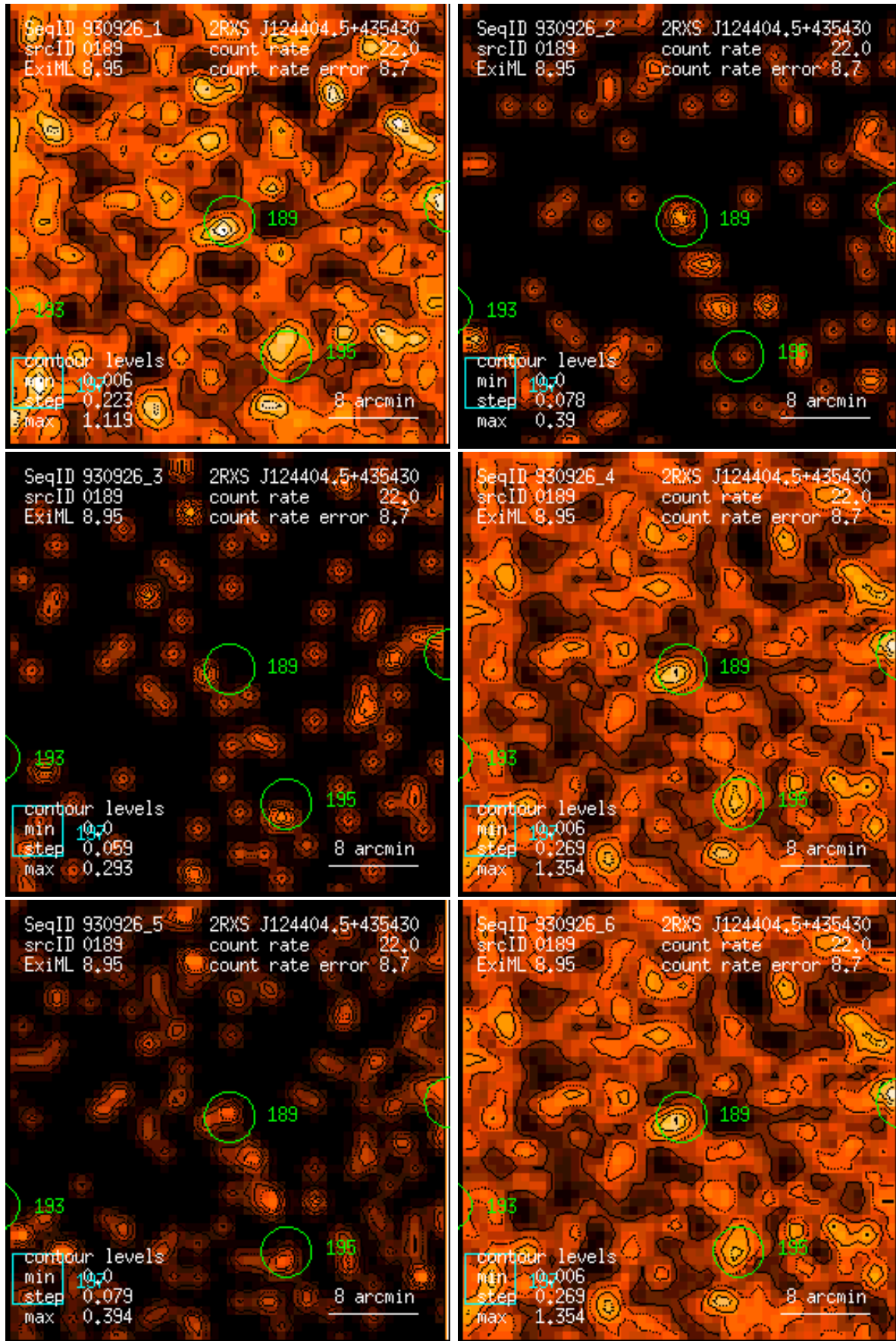
Figure 189: RASS 930926: detection 0189: band rate images, Gaussian filter: (1) PSPC channels 11 – 41, (2) 52 – 90, (3) 91 – 201, (4) 11 – 235, (5) 52 – 201, (6) 11 – 201. Broad band rates in counts/ks. Band rate contour levels in counts/ks/arcmin 2 .
