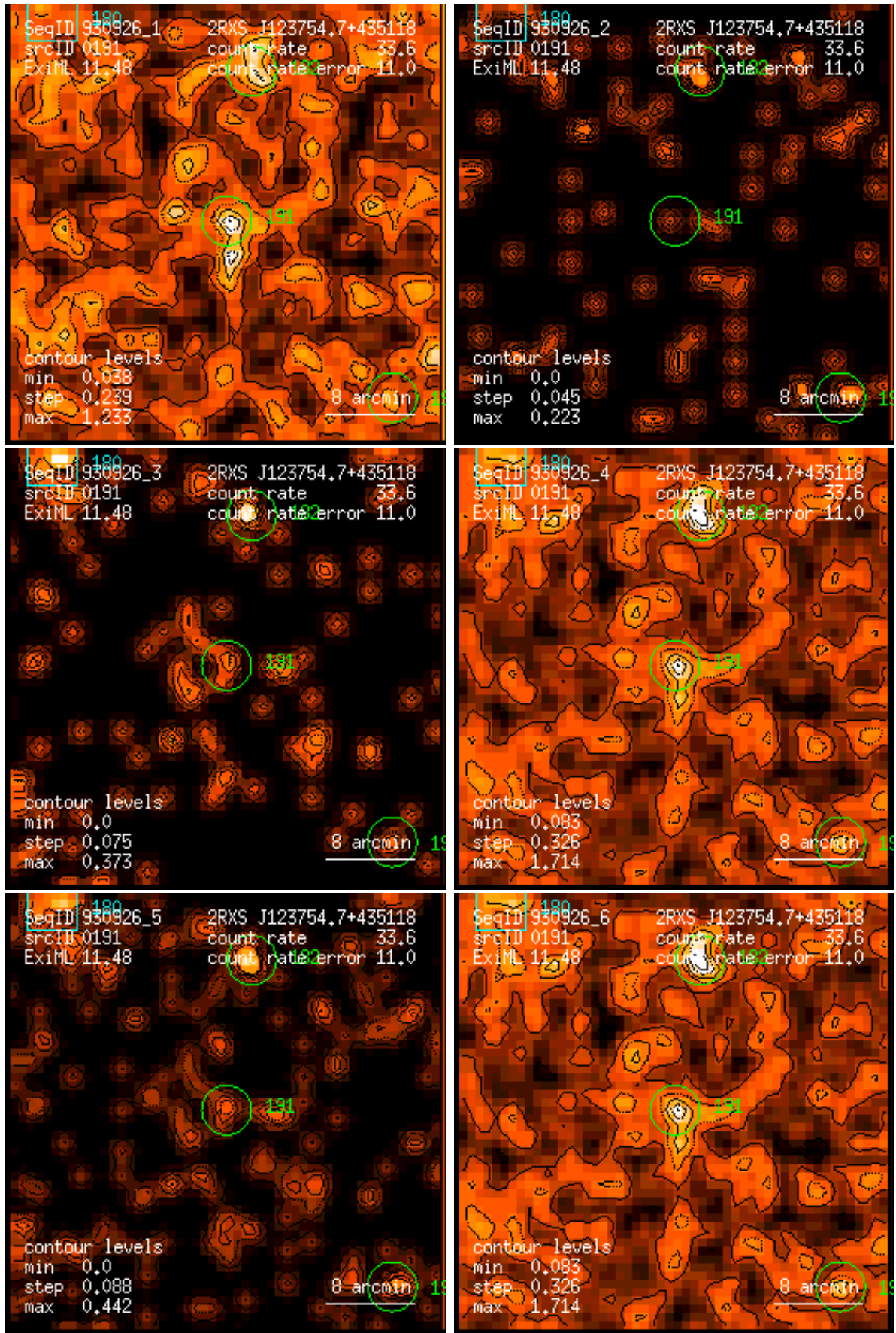
Figure 191: RASS 930926: detection 0191: band rate images, Gaussian filter: (1) PSPC channels 11 – 41, (2) 52 – 90, (3) 91 – 201, (4) 11 – 235, (5) 52 – 201, (6) 11 – 201. Broad band rates in counts/ks. Band rate contour levels in counts/ks/arcmin 2 .
