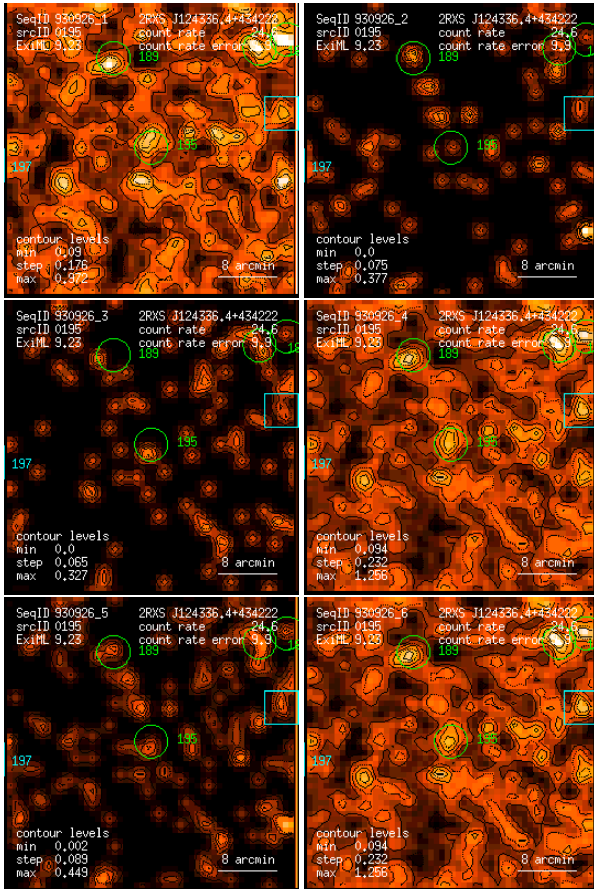
Figure 195: RASS 930926: detection 0195: band rate images, Gaussian filter: (1) PSPC channels 11 – 41, (2) 52 – 90, (3) 91 – 201, (4) 11 – 235, (5) 52 – 201, (6) 11 – 201. Broad band rates in counts/ks. Band rate contour levels in counts/ks/arcmin 2 .
