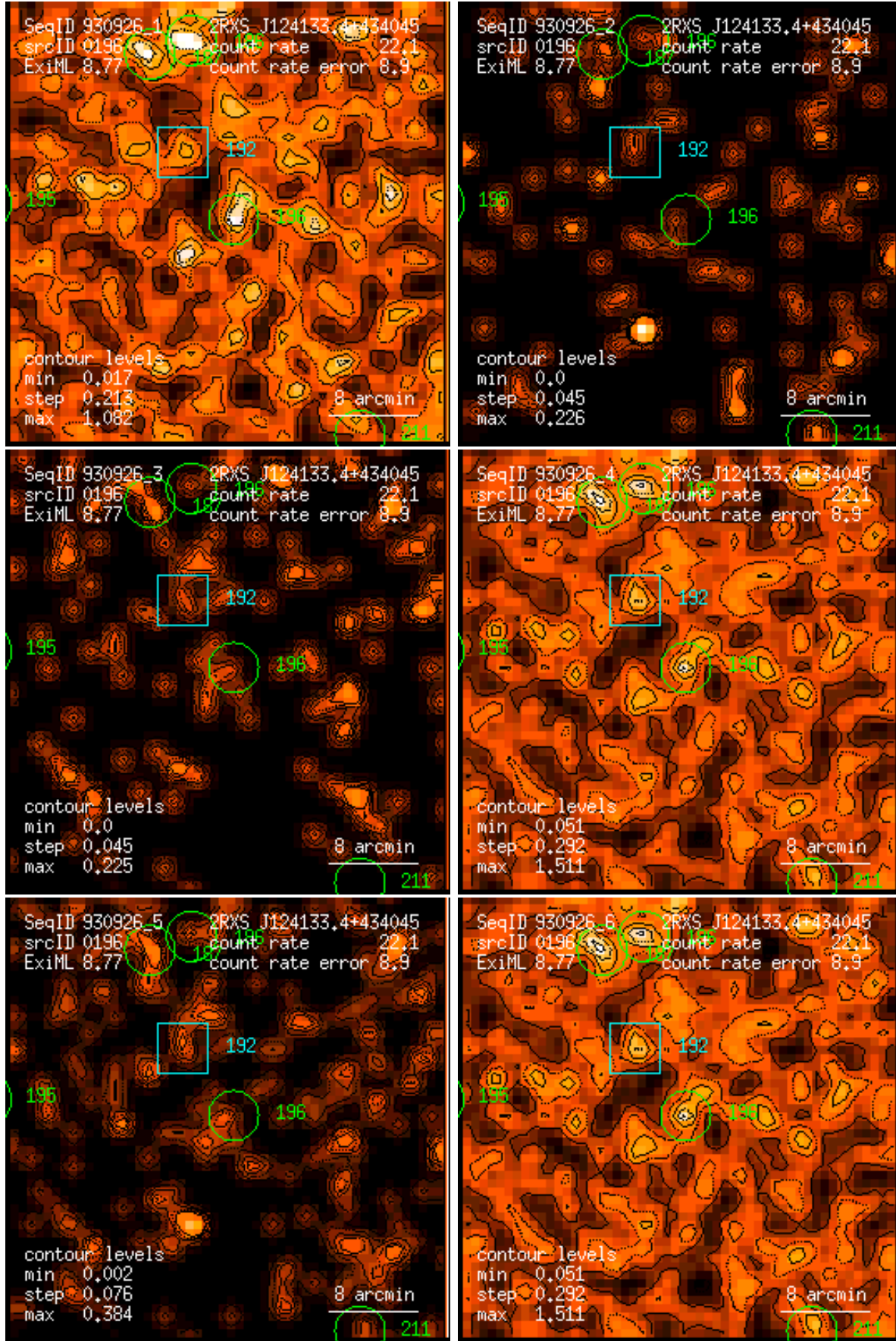
Figure 196: RASS 930926: detection 0196: band rate images, Gaussian filter: (1) PSPC channels 11 – 41, (2) 52 – 90, (3) 91 – 201, (4) 11 – 235, (5) 52 – 201, (6) 11 – 201. Broad band rates in counts/ks. Band rate contour levels in counts/ks/arcmin 2 .
