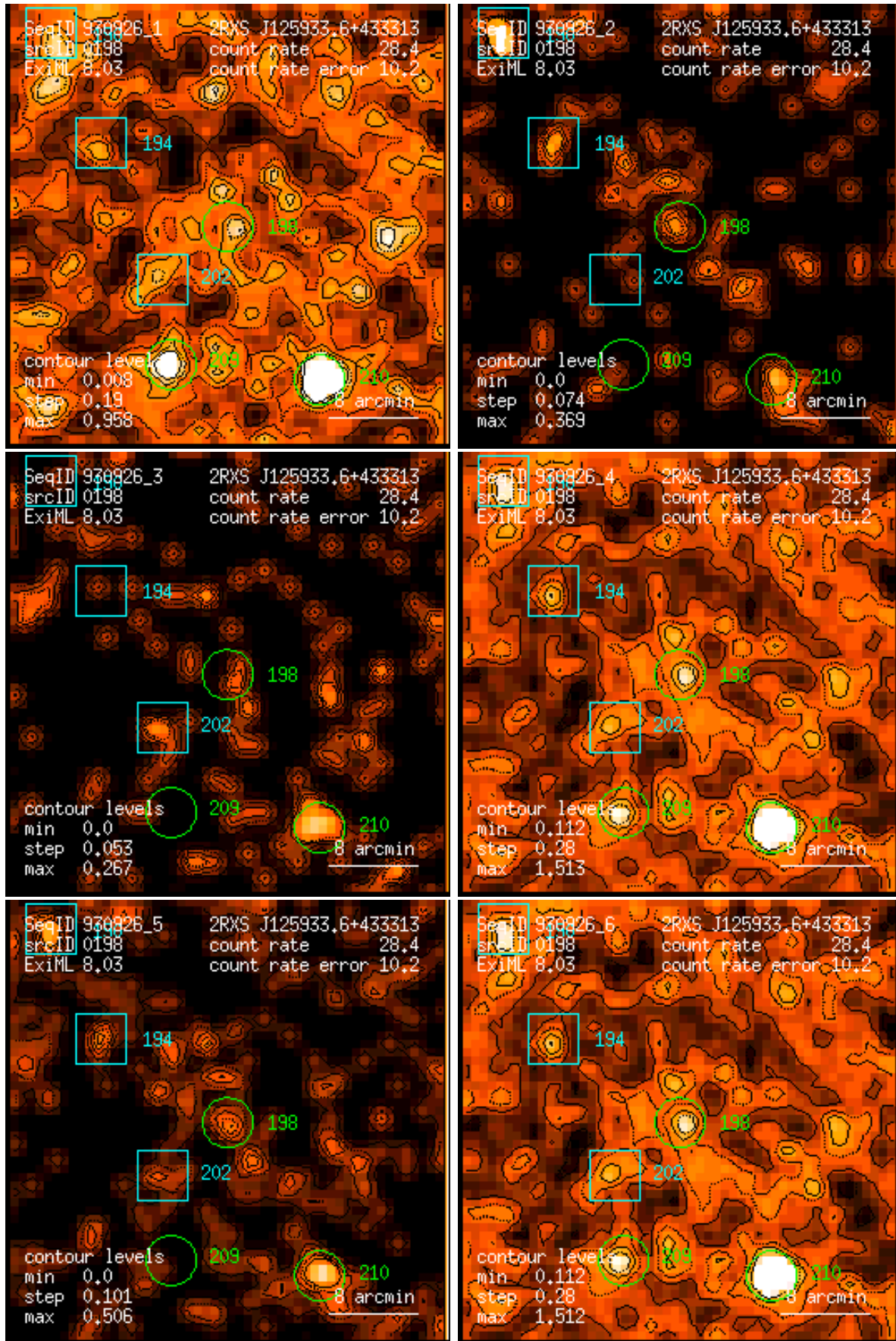
Figure 198: RASS 930926: detection 0198: band rate images, Gaussian filter: (1) PSPC channels 11 – 41, (2) 52 – 90, (3) 91 – 201, (4) 11 – 235, (5) 52 – 201, (6) 11 – 201. Broad band rates in counts/ks. Band rate contour levels in counts/ks/arcmin 2 .
