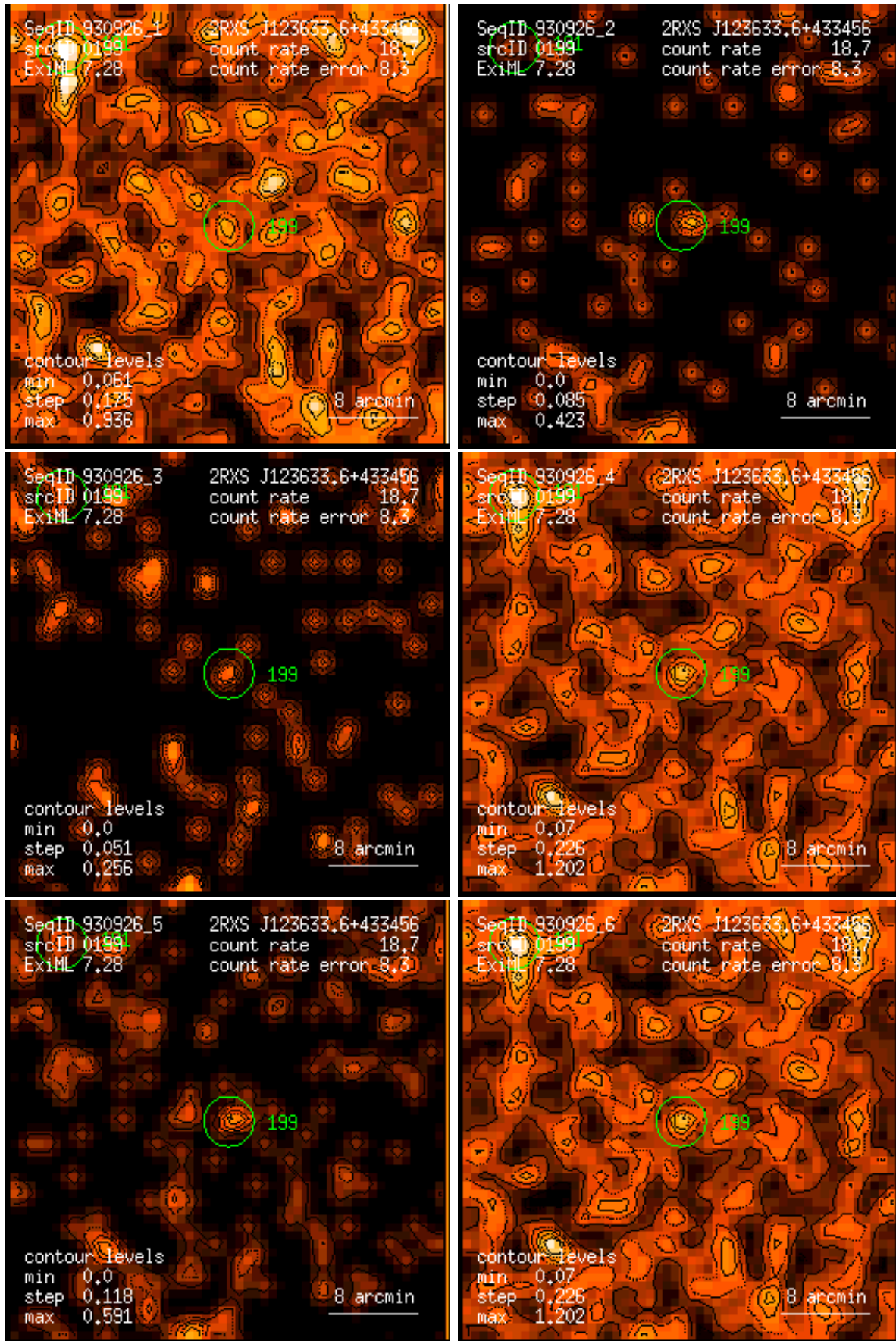
Figure 199: RASS 930926: detection 0199: band rate images, Gaussian filter: (1) PSPC channels 11 – 41, (2) 52 – 90, (3) 91 – 201, (4) 11 – 235, (5) 52 – 201, (6) 11 – 201. Broad band rates in counts/ks. Band rate contour levels in counts/ks/arcmin 2 .
